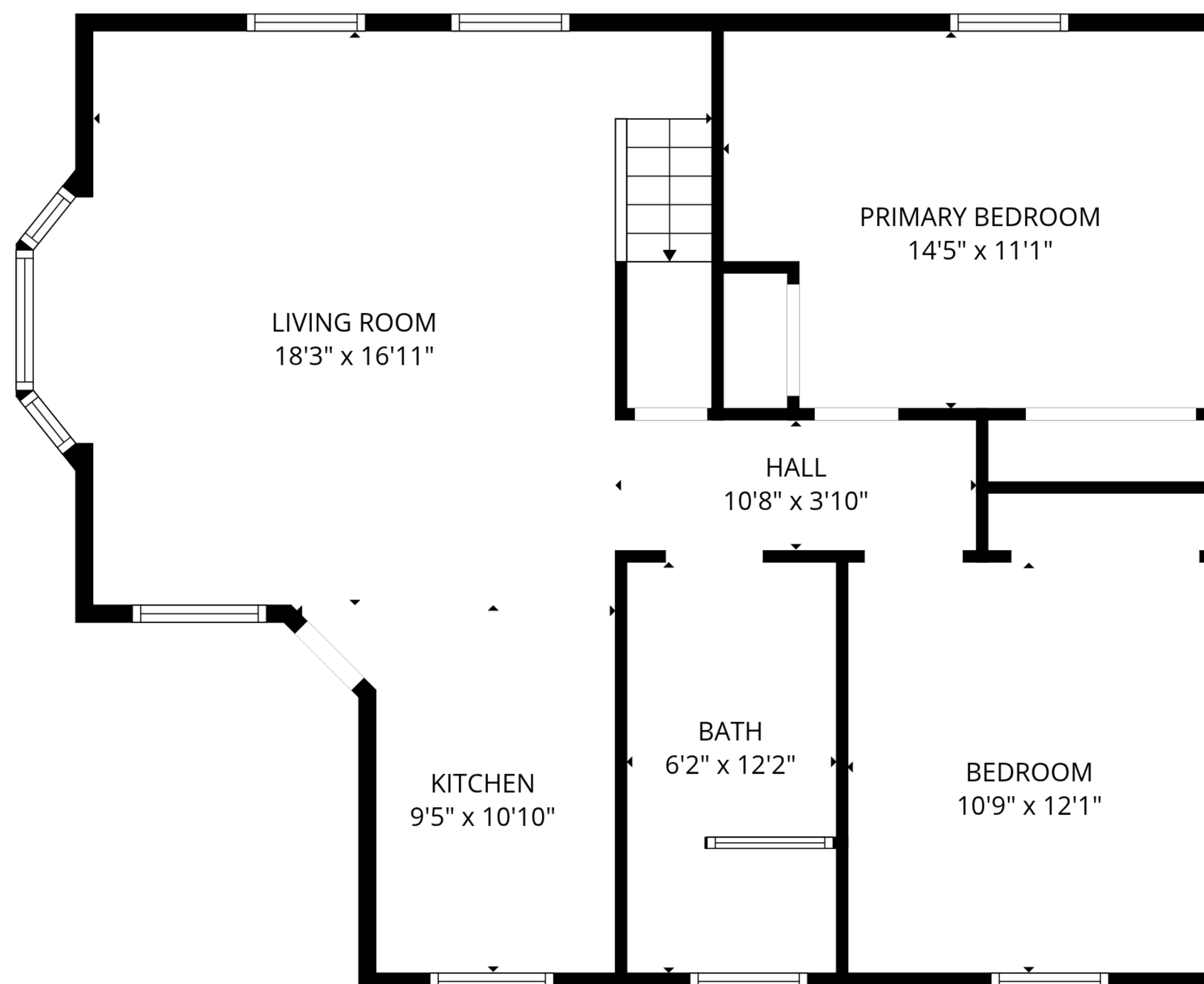
1st floor
