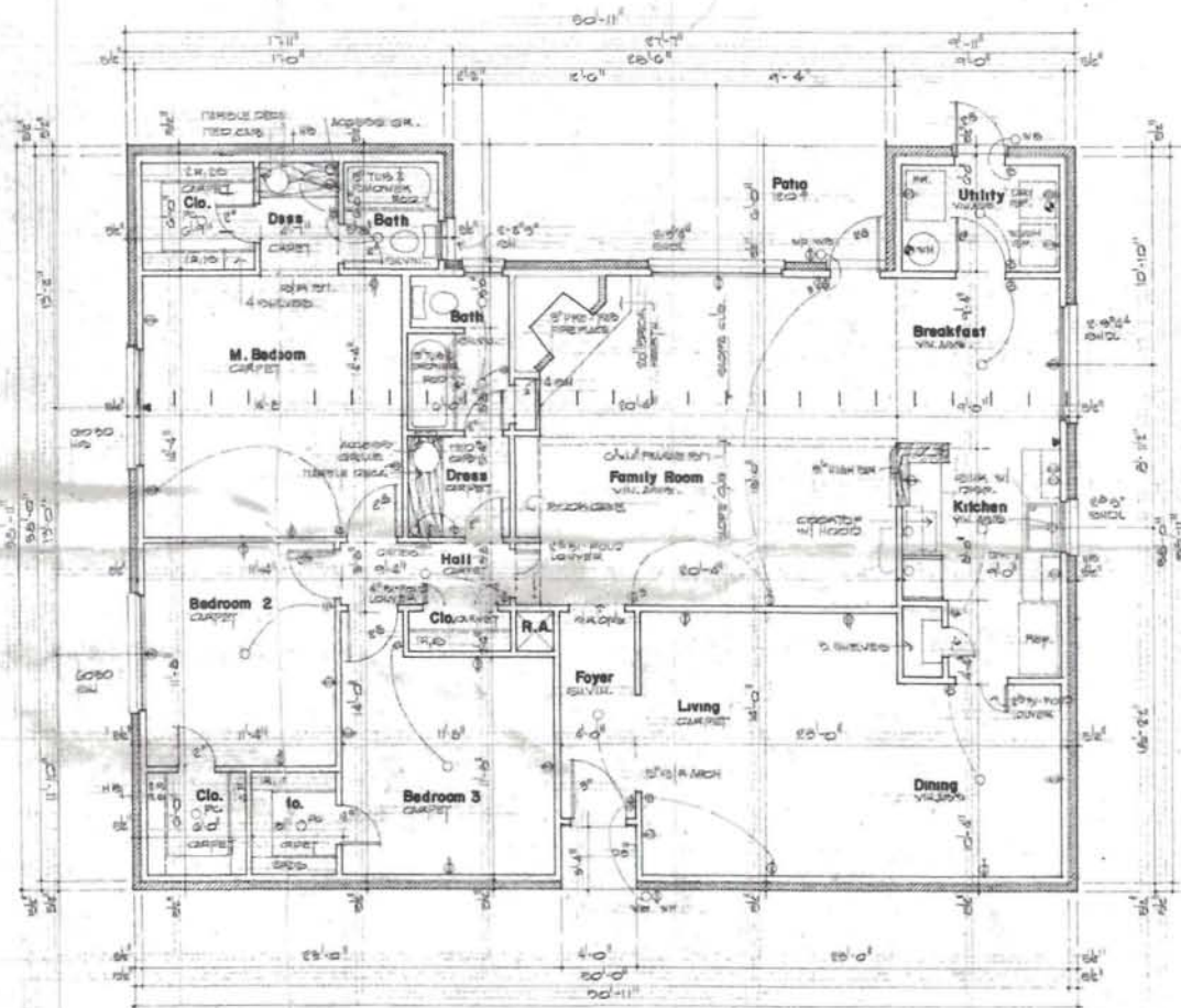
FLOOR PLAN 14' x 12'
