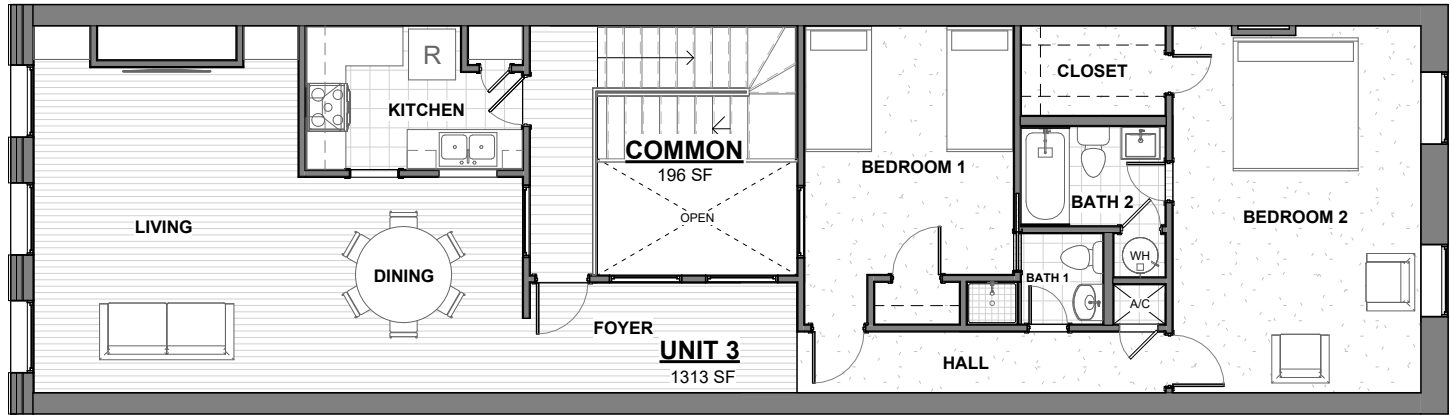
3 THIRD FLOOR - 1509 SF 1" = 10'-0"
