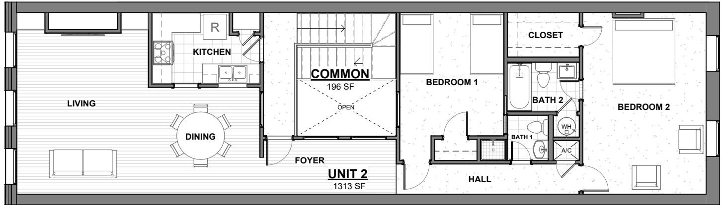
2 SECOND FLOOR - 1509 SF 1" = 10'-0"
