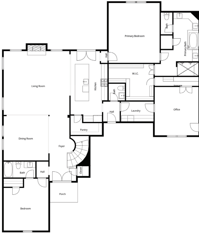
1st Floor
