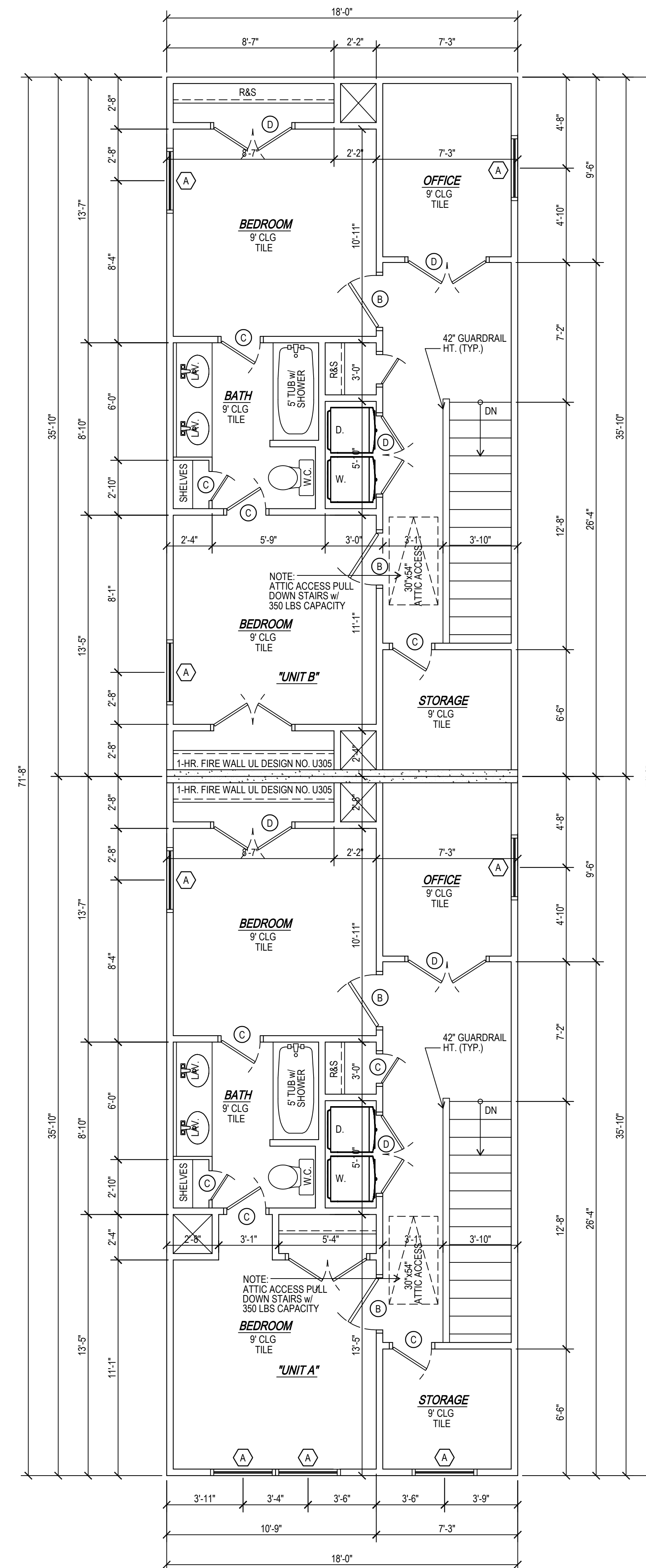
FLOOR PLAN- 2ND FLOOR
