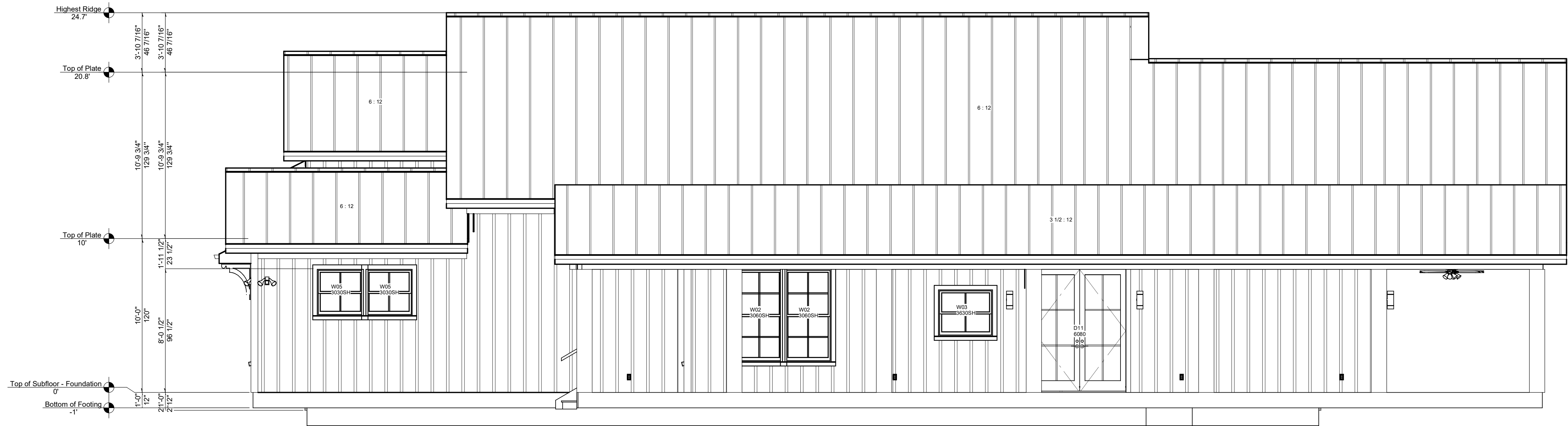
Exterior Elevation Right
