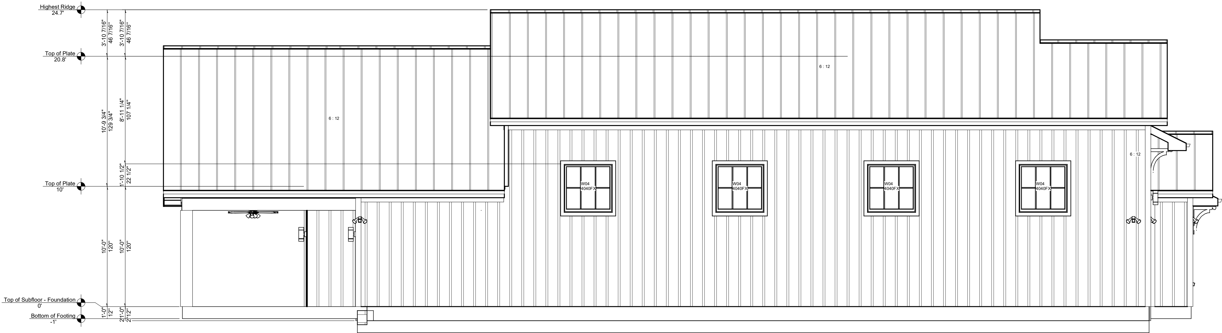
Exterior Elevation Left
