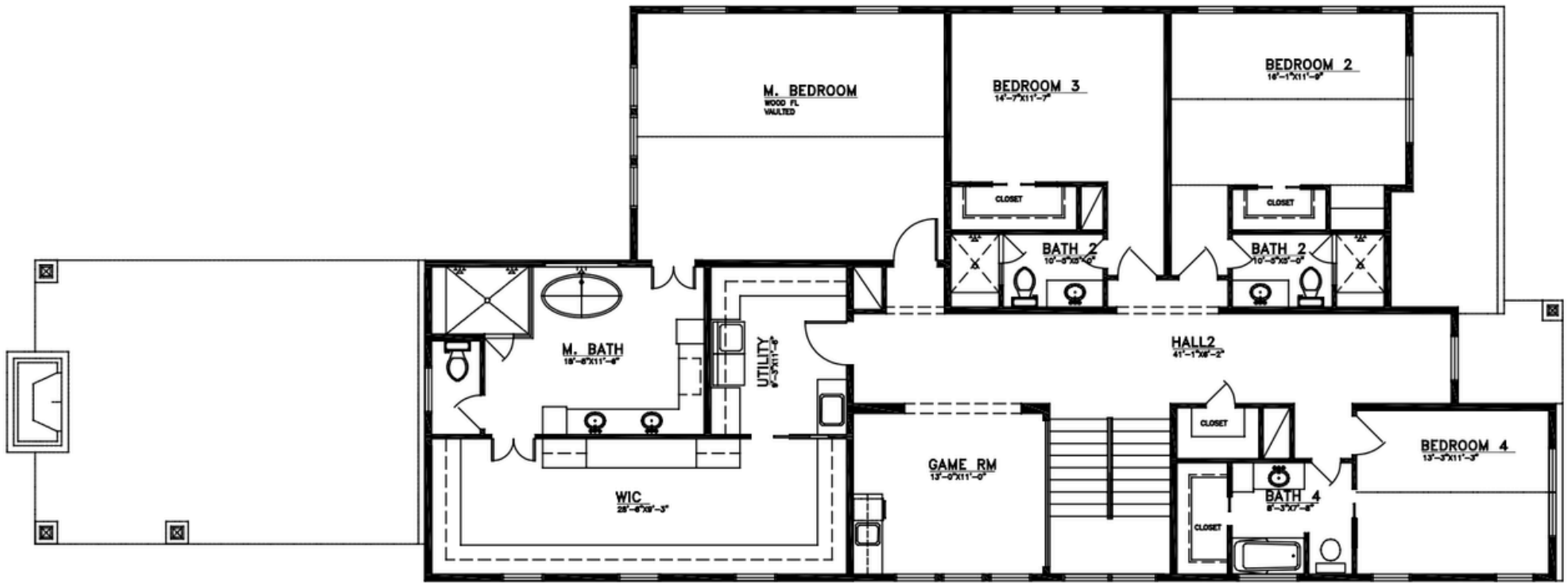
5451 RICHMOND AVE. 2ND FLOOR PLAN
