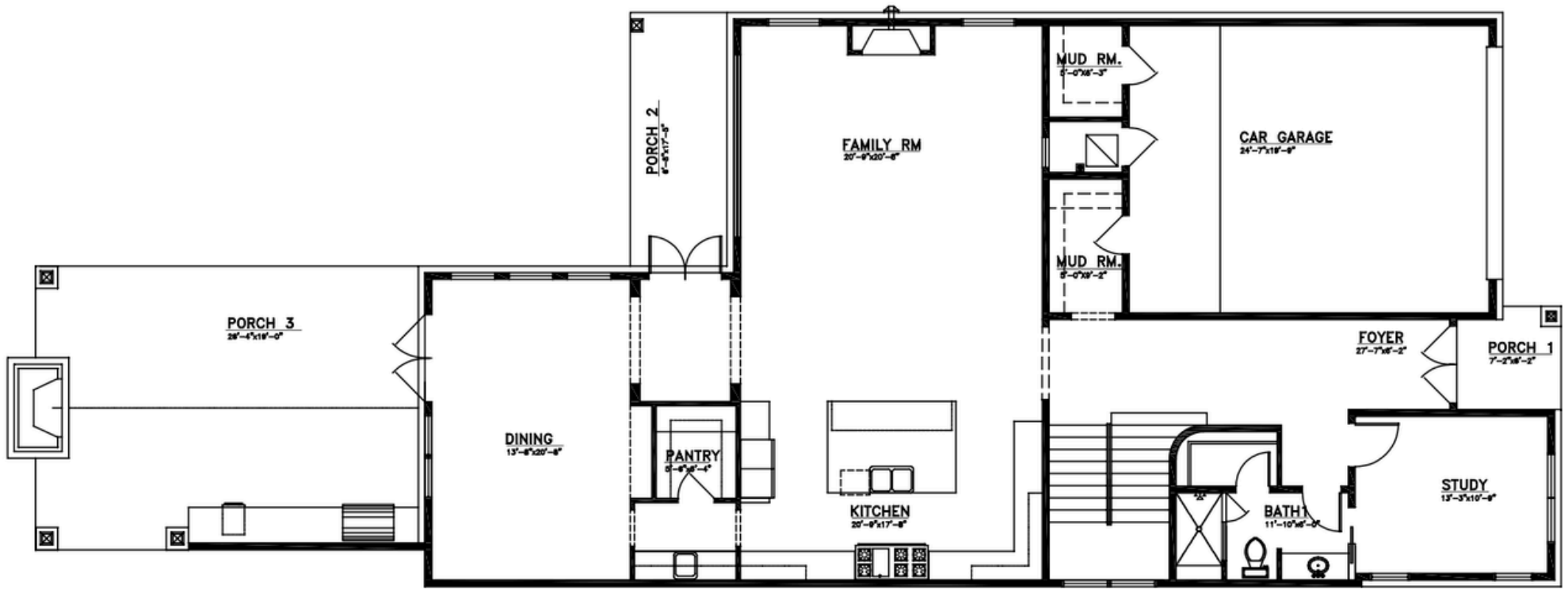
5451 RICHMOND AVE. 1ST FLOOR PLAN
