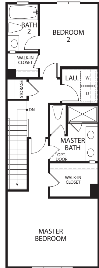
THIRD FLOOR
