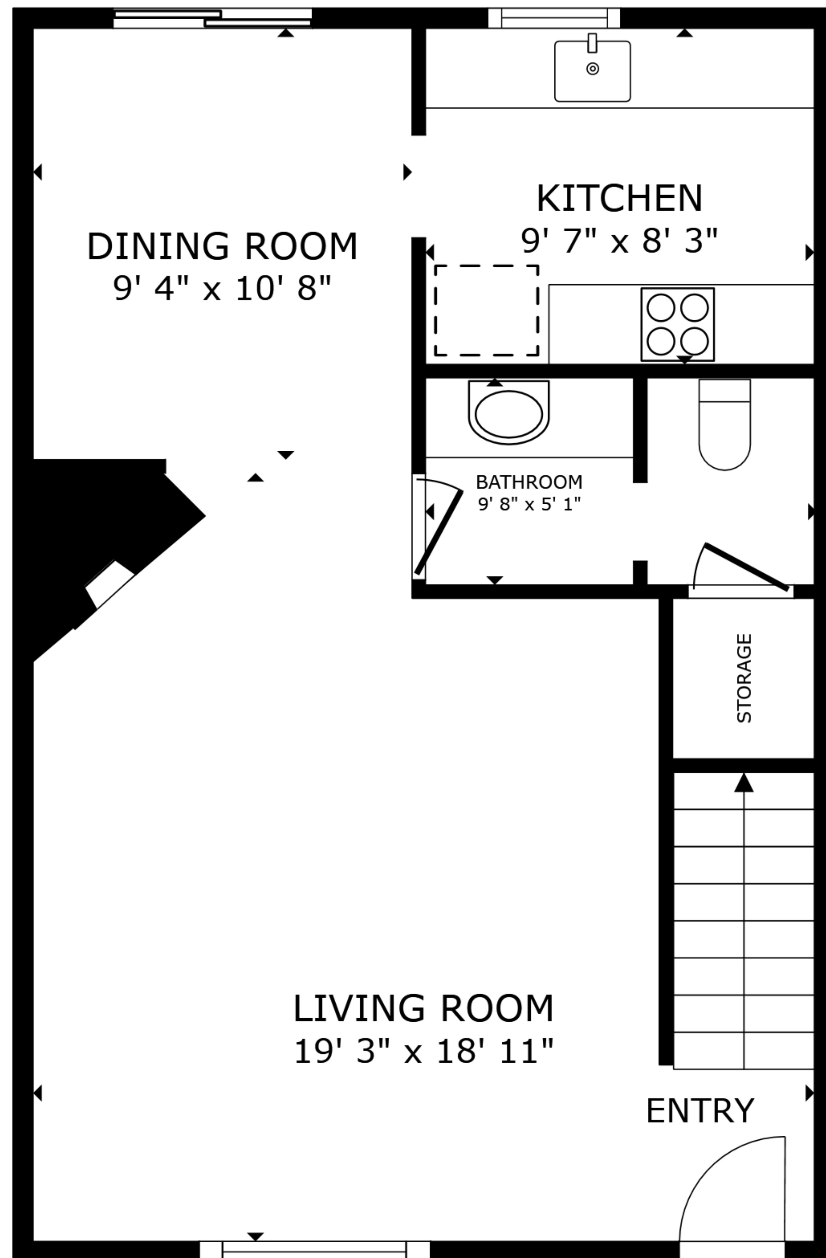
FLOOR 1
