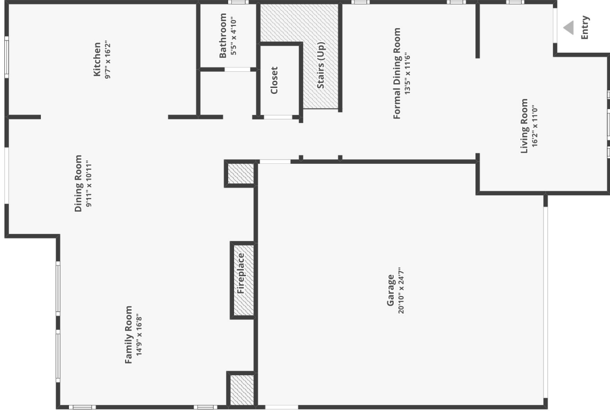
FLOOR 1
