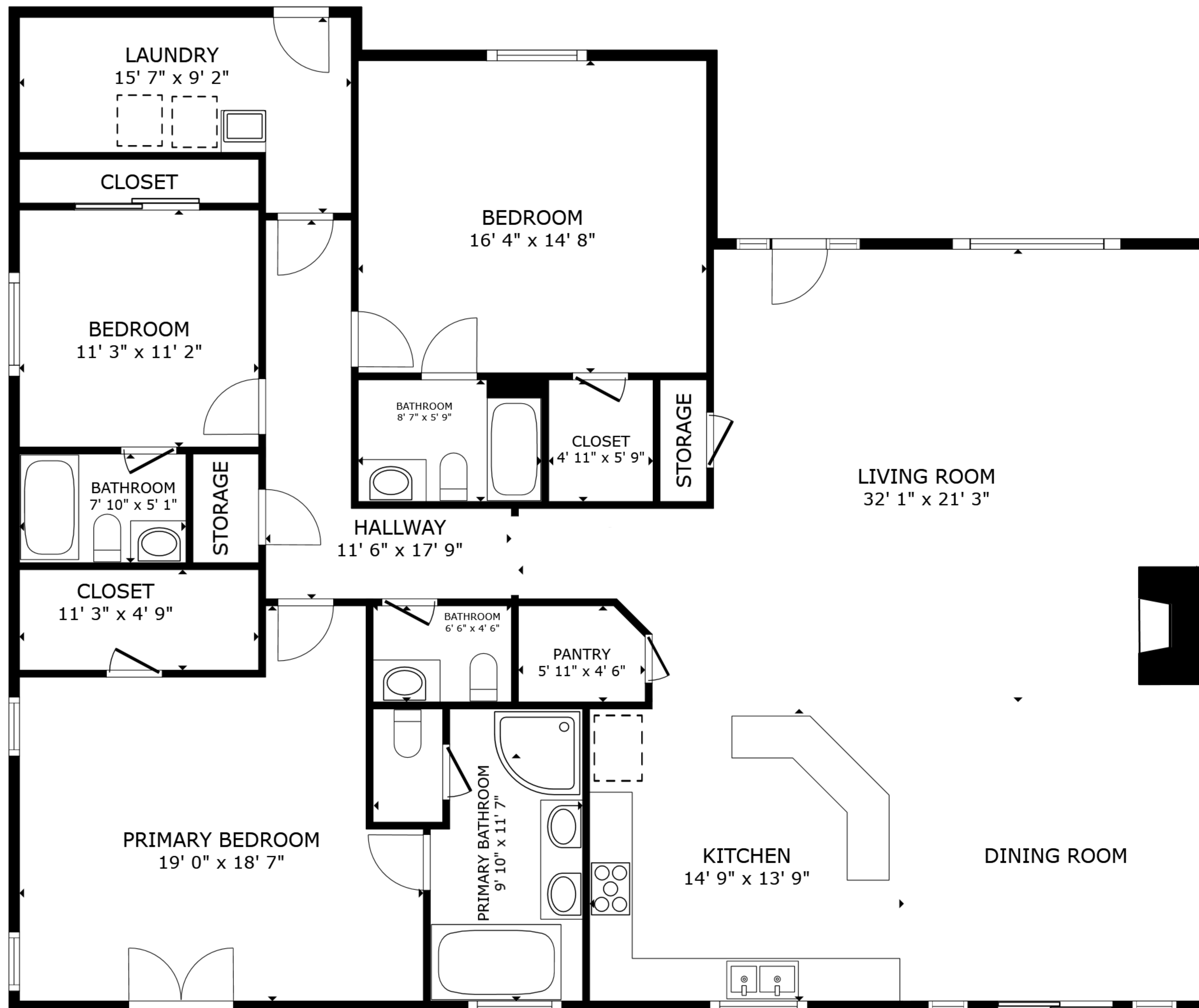
FLOOR PLAN
