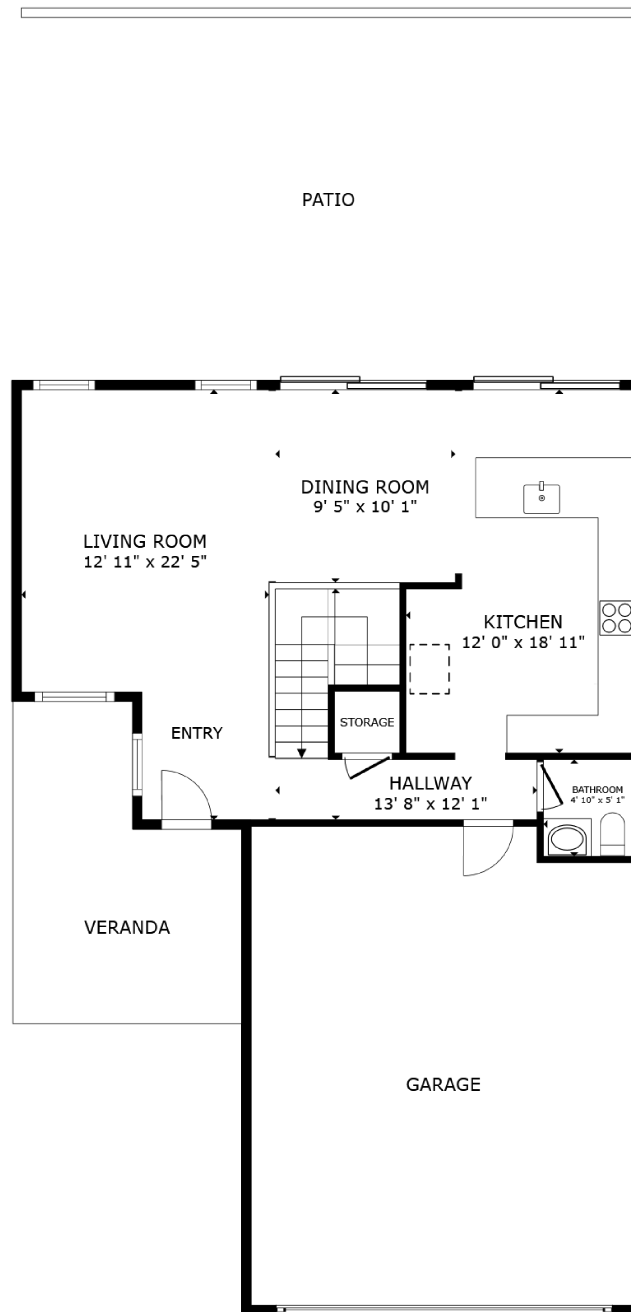
FLOOR 1
