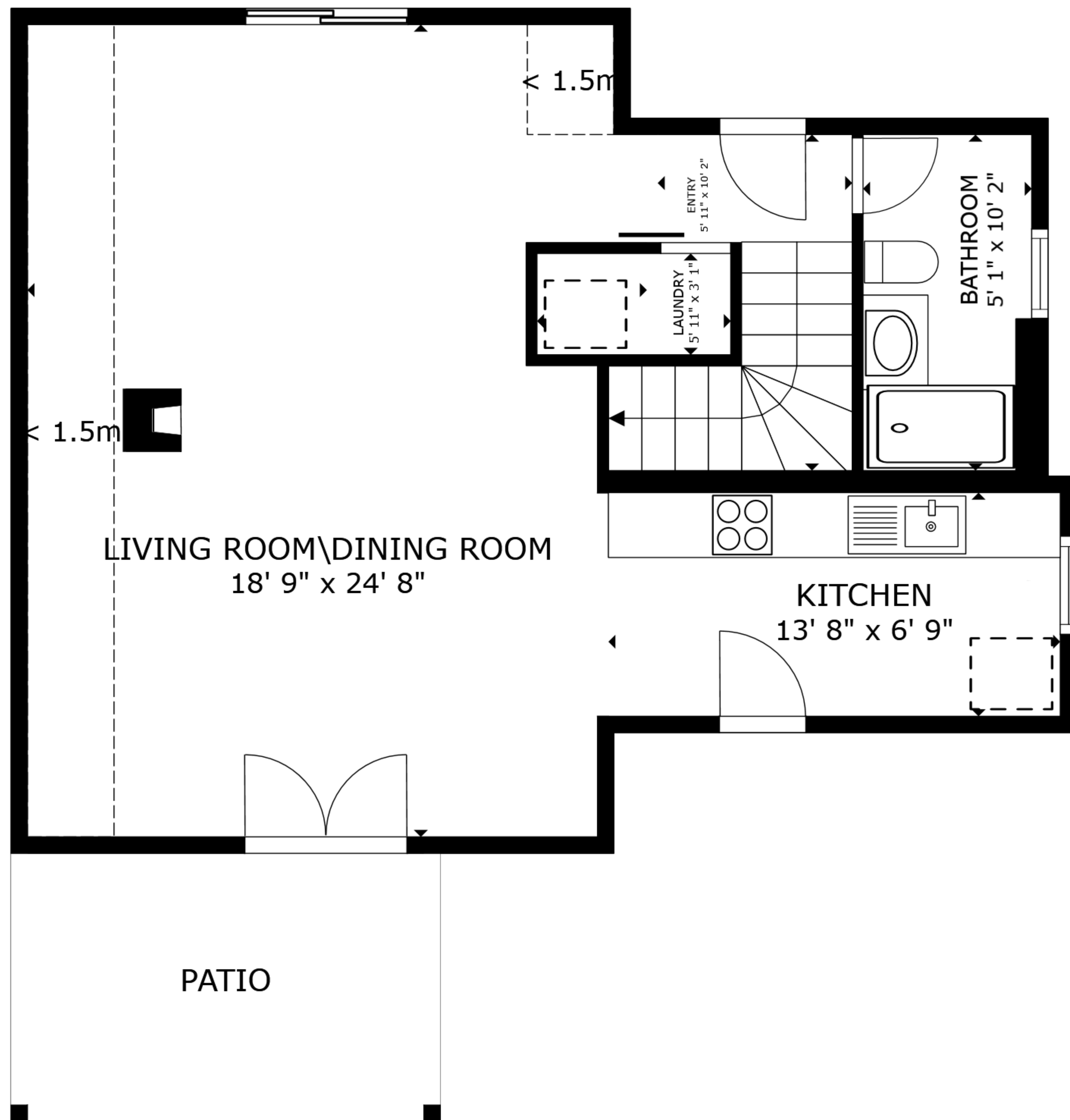
FLOOR 1
