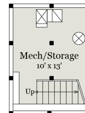
LOWER LEVEL
