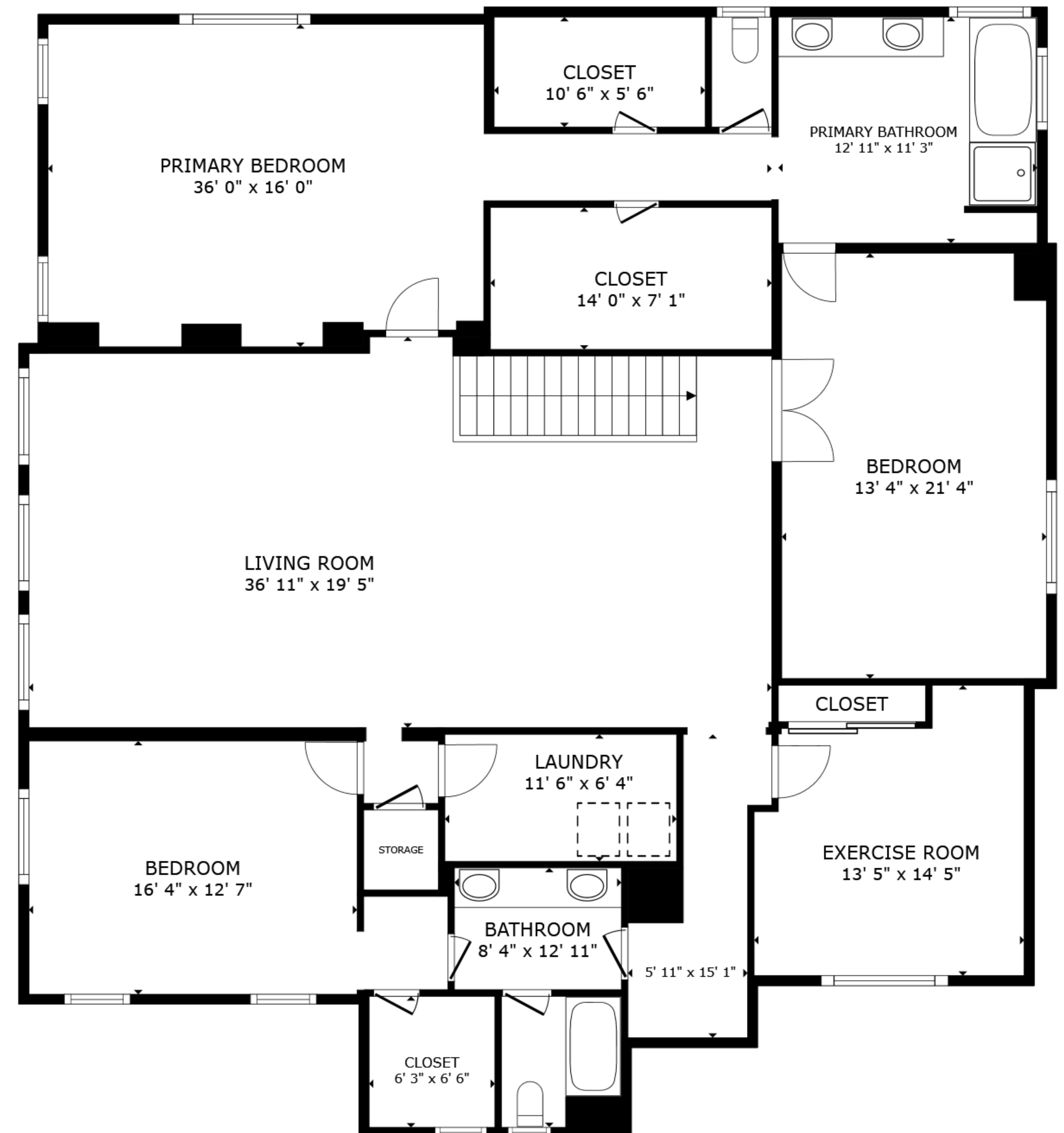
FLOOR 2
