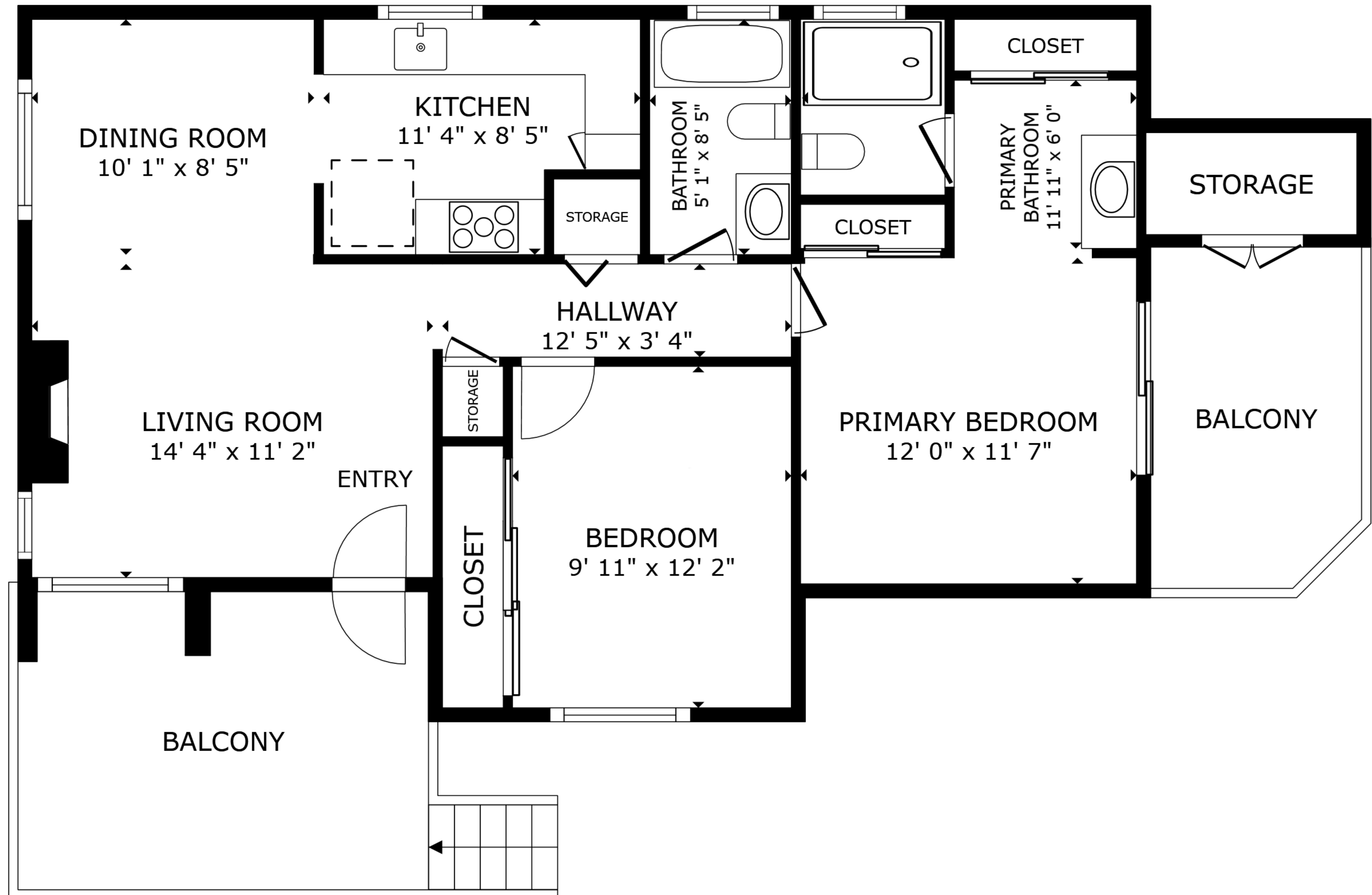
FLOOR PLAN
