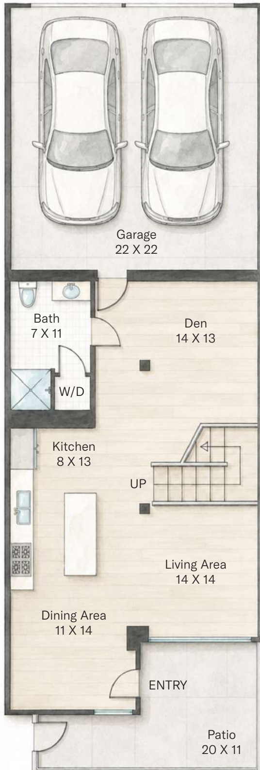
Main Level
