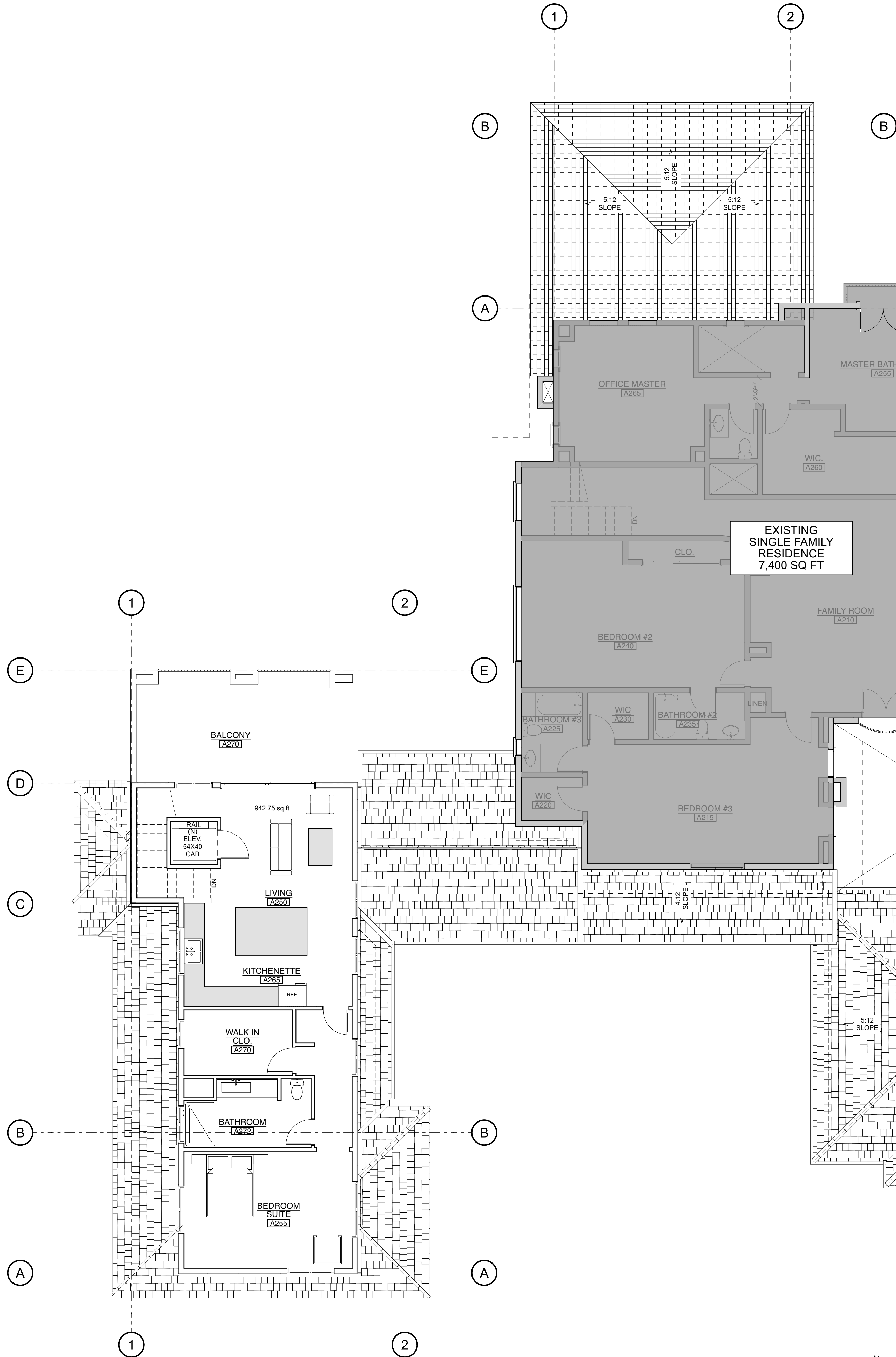
A PARTIAL SECOND FLOOR REFERENCE PLAN SCALE: 3/16" = 1'-0"
