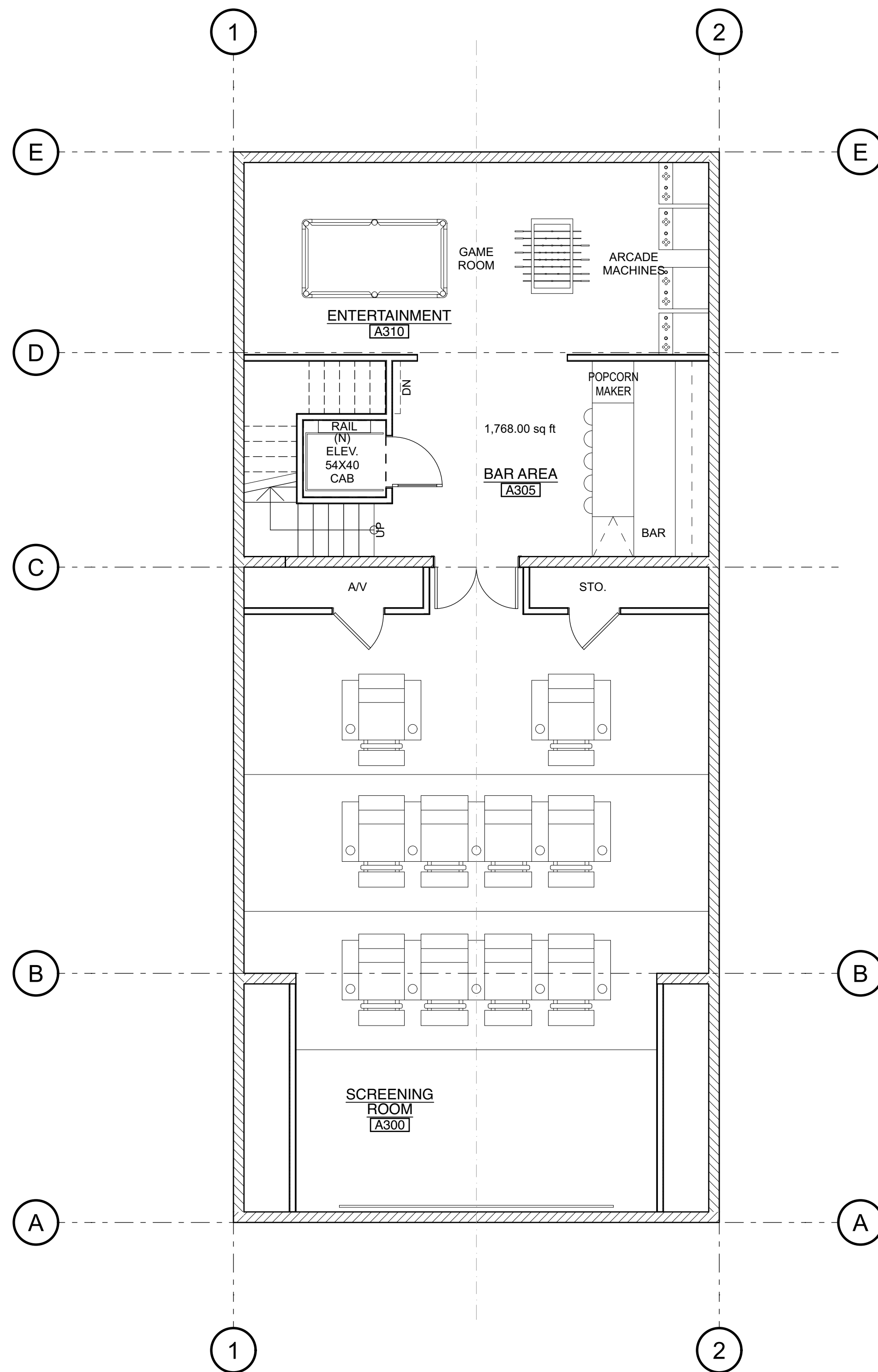
A PARTIAL BASEMENT FLOOR REFERENCE PLAN SCALE: 3/16" = 1'-0"
