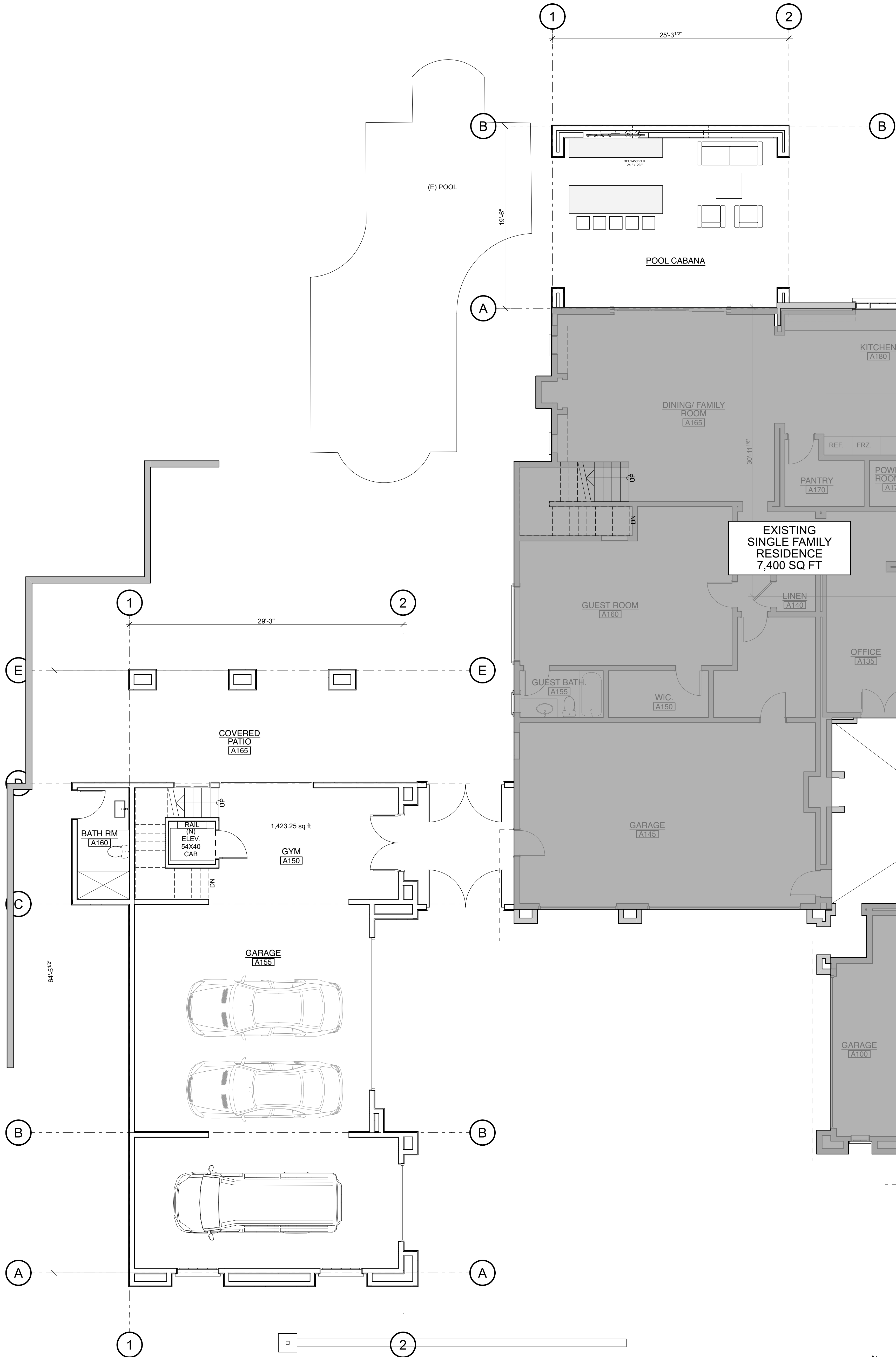
B PARTIAL FIRST FLOOR REFERENCE PLAN SCALE: 3/16" = 1'-0"
