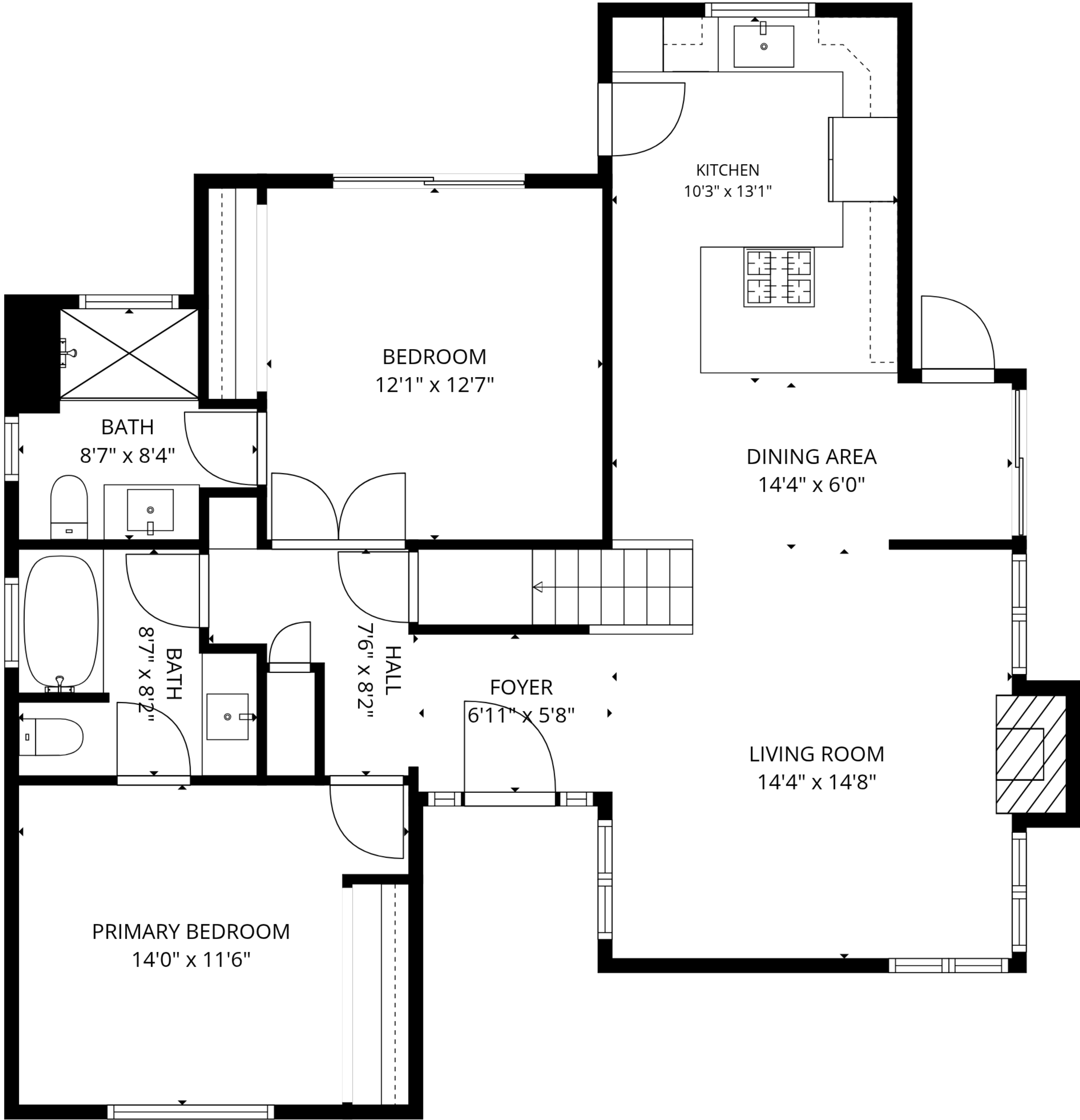
1st floor
