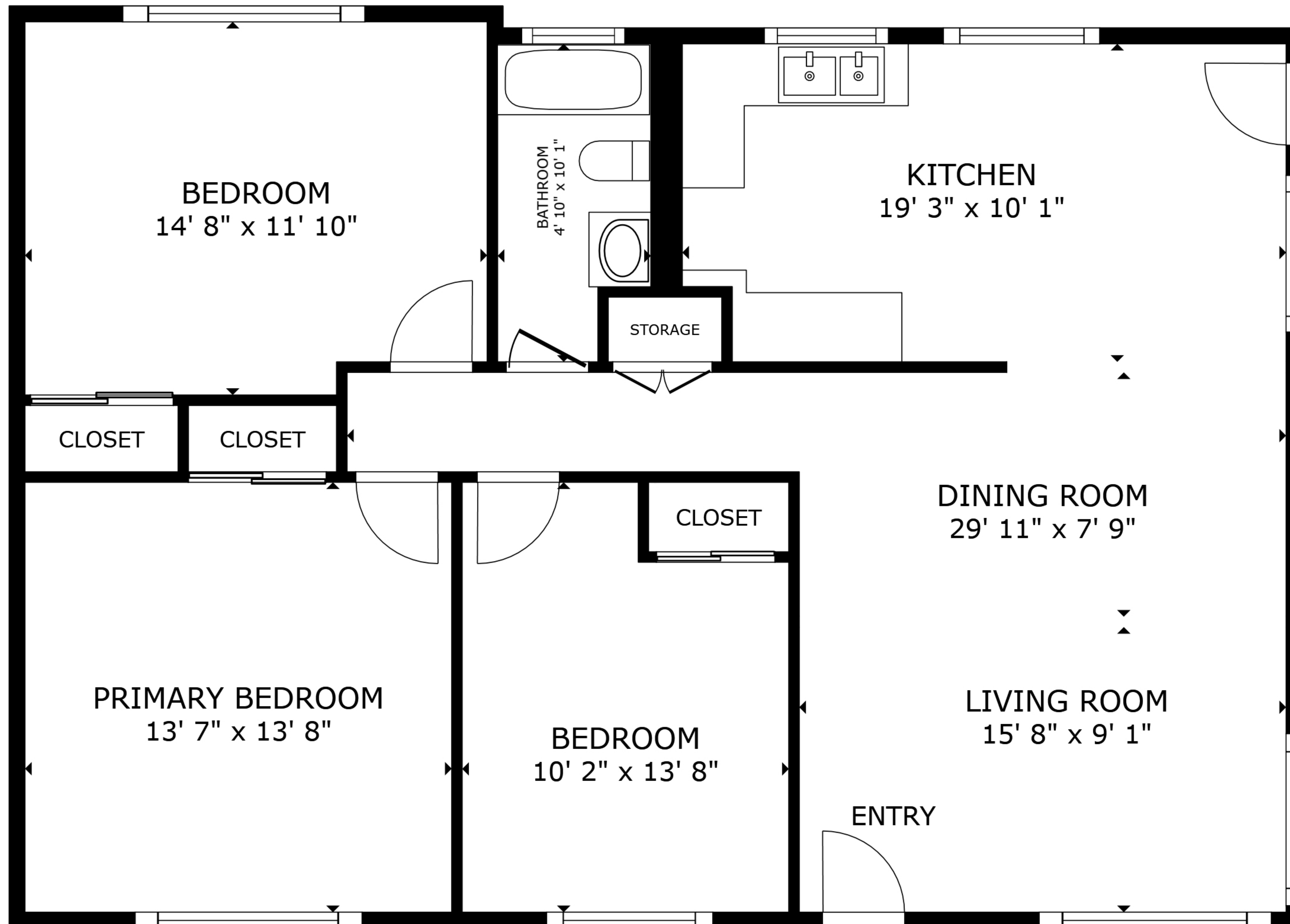
FLOOR PLAN
