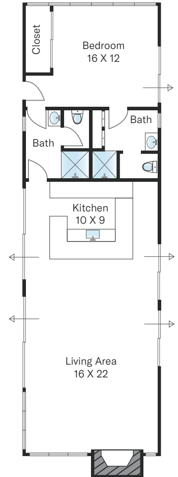
Main Level - Pool House
