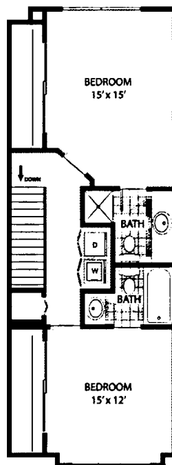
UPPER FLOOR
