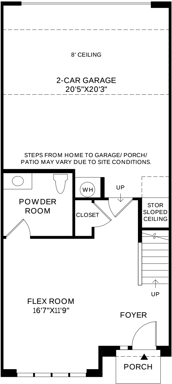
FIRST FLOOR 9' CEILING HEIGHT
