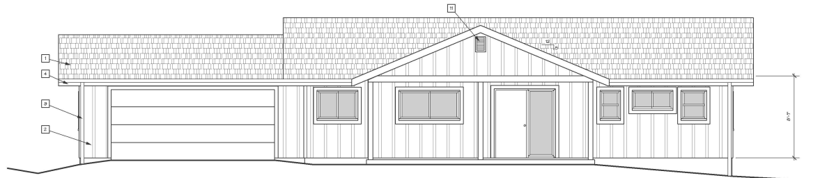
FRONT (NORTH) ELEVATION SCALE 1/4" = 1'-0"
