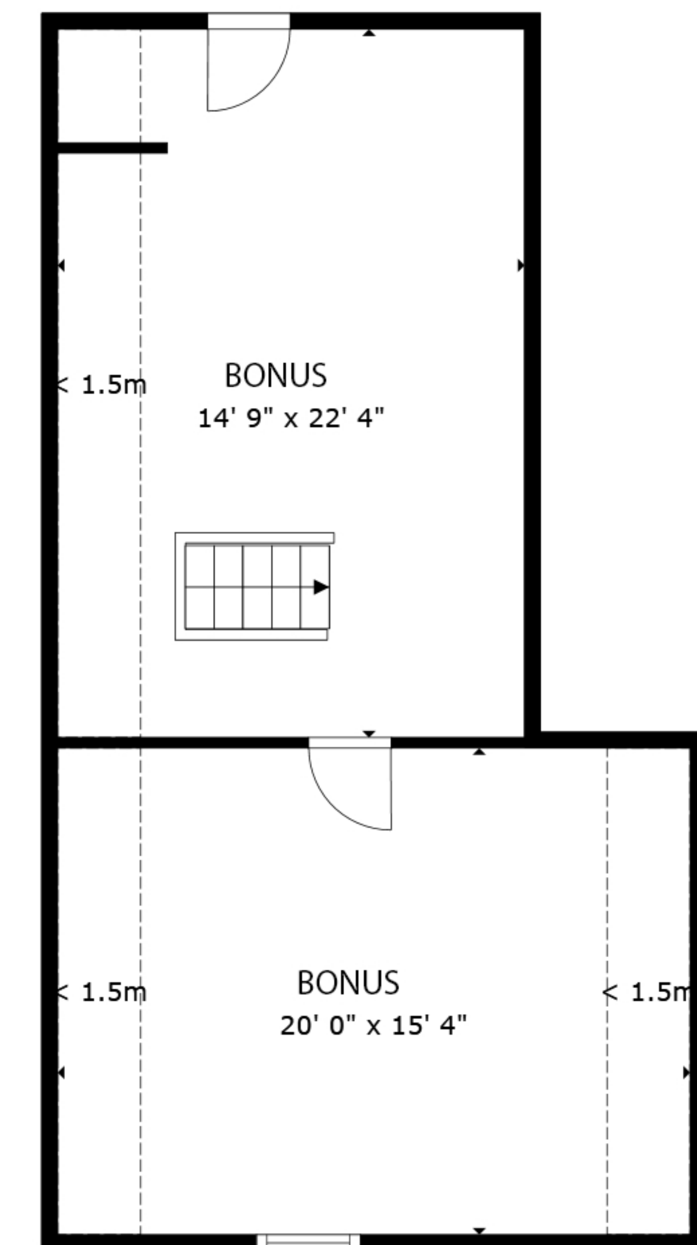
FLOOR 2
