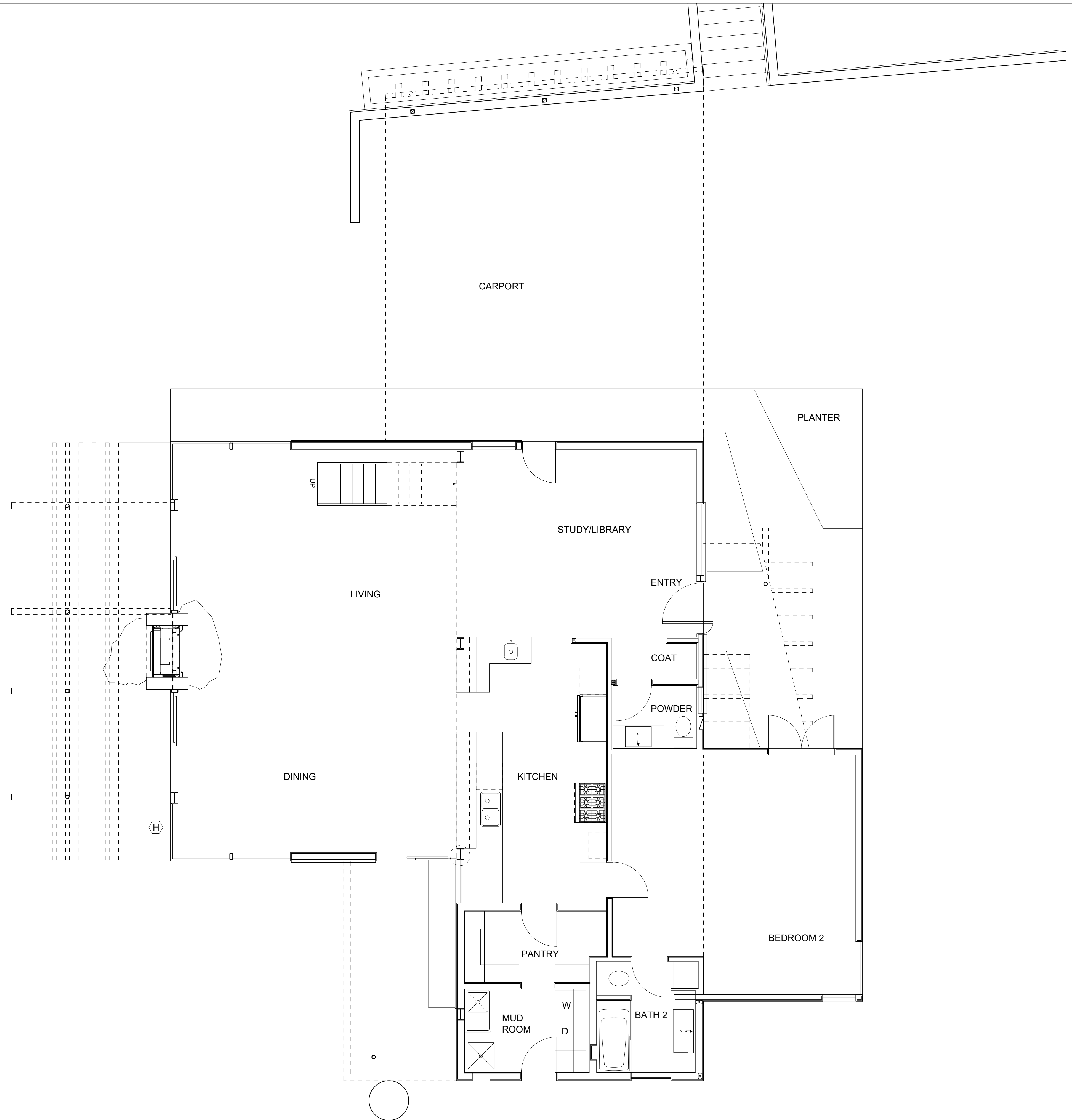
PARADISE LODGE 1ST FLOOR PLAN
