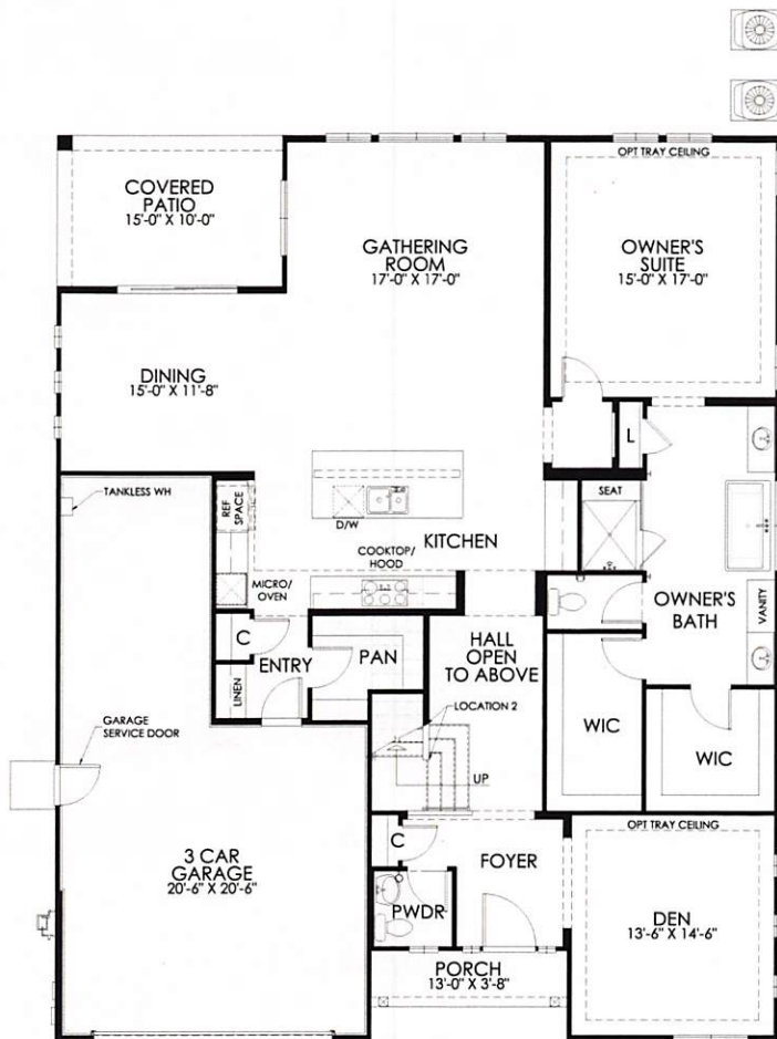
FIRST FLOOR
