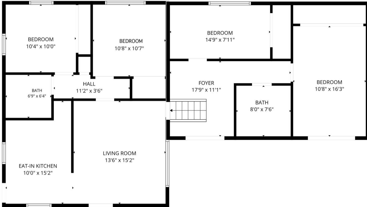
UPPER FLOOR
