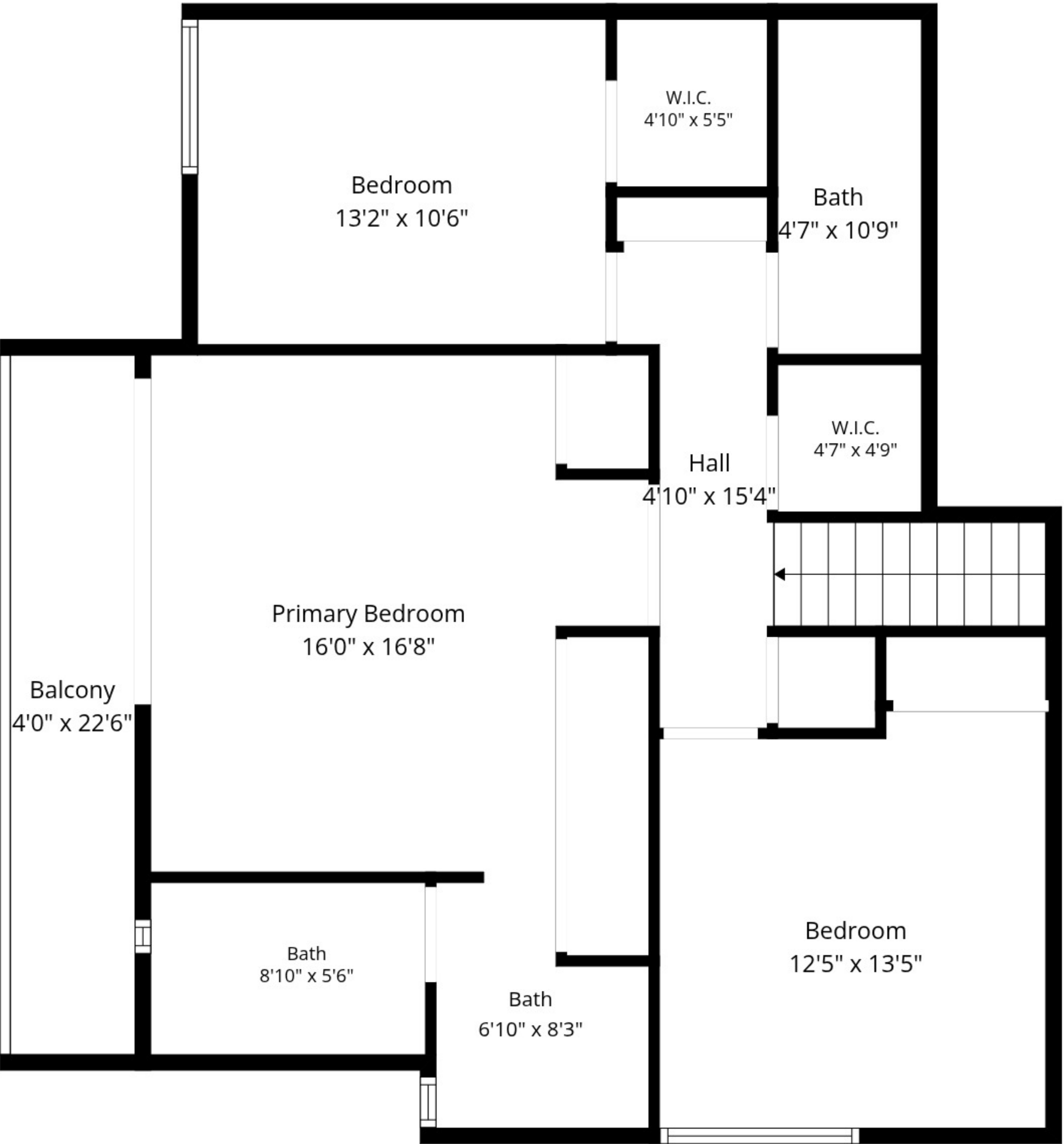
3rd Floor
