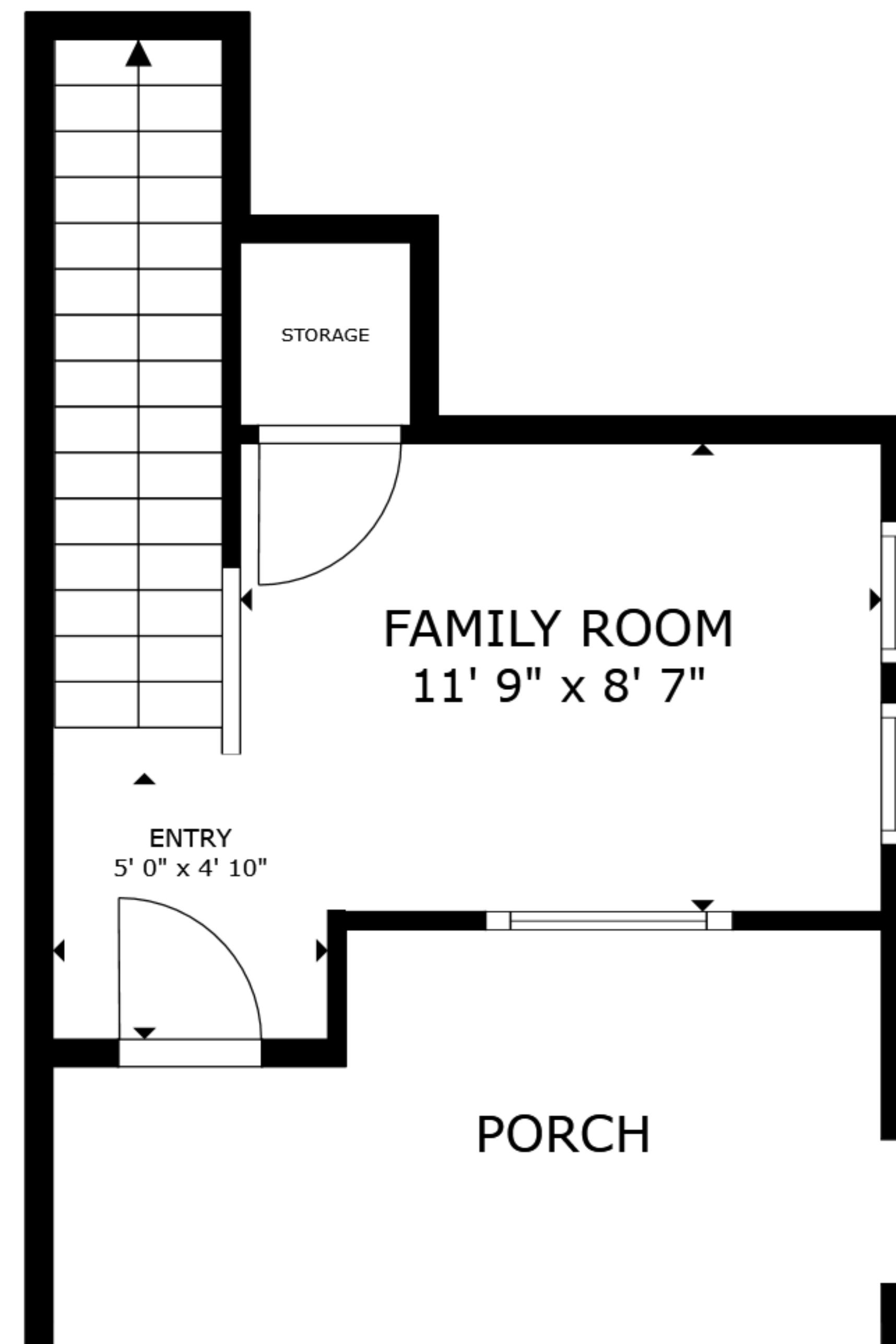
FLOOR 1
