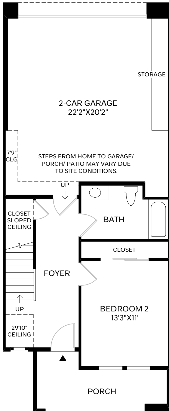
FIRST FLOOR 9' CEILING HEIGHT
