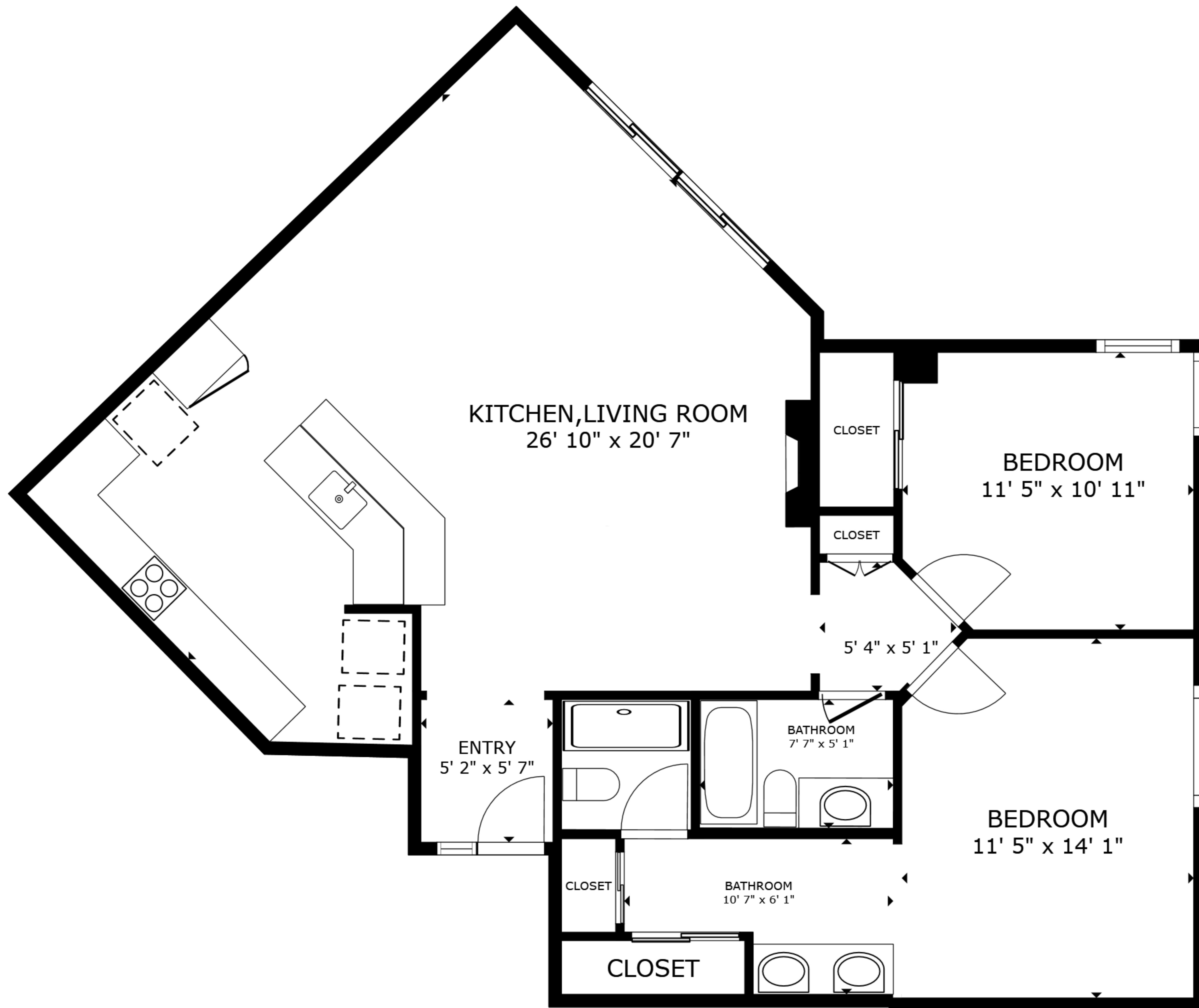
FLOOR PLAN
