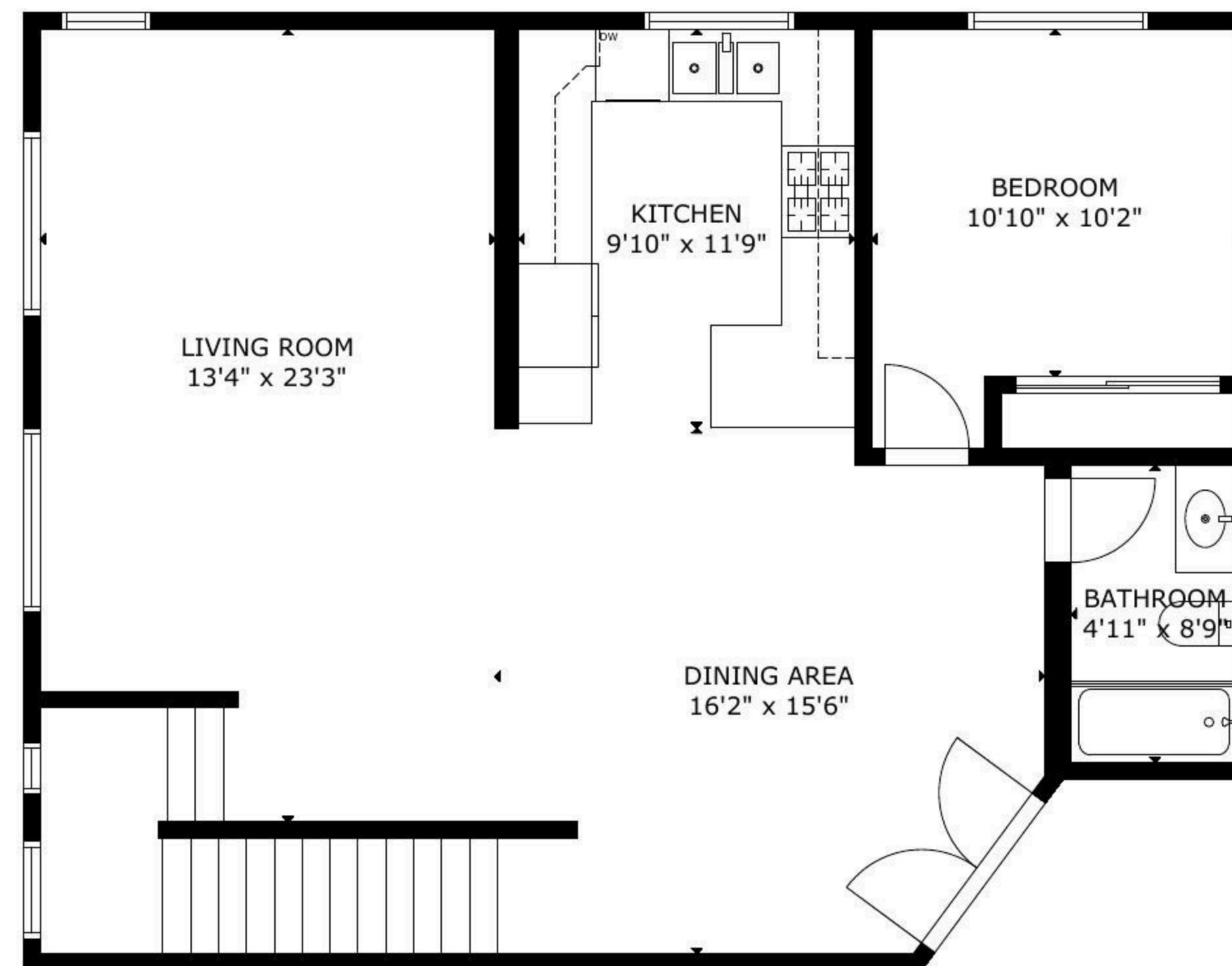
FLOOR 2
