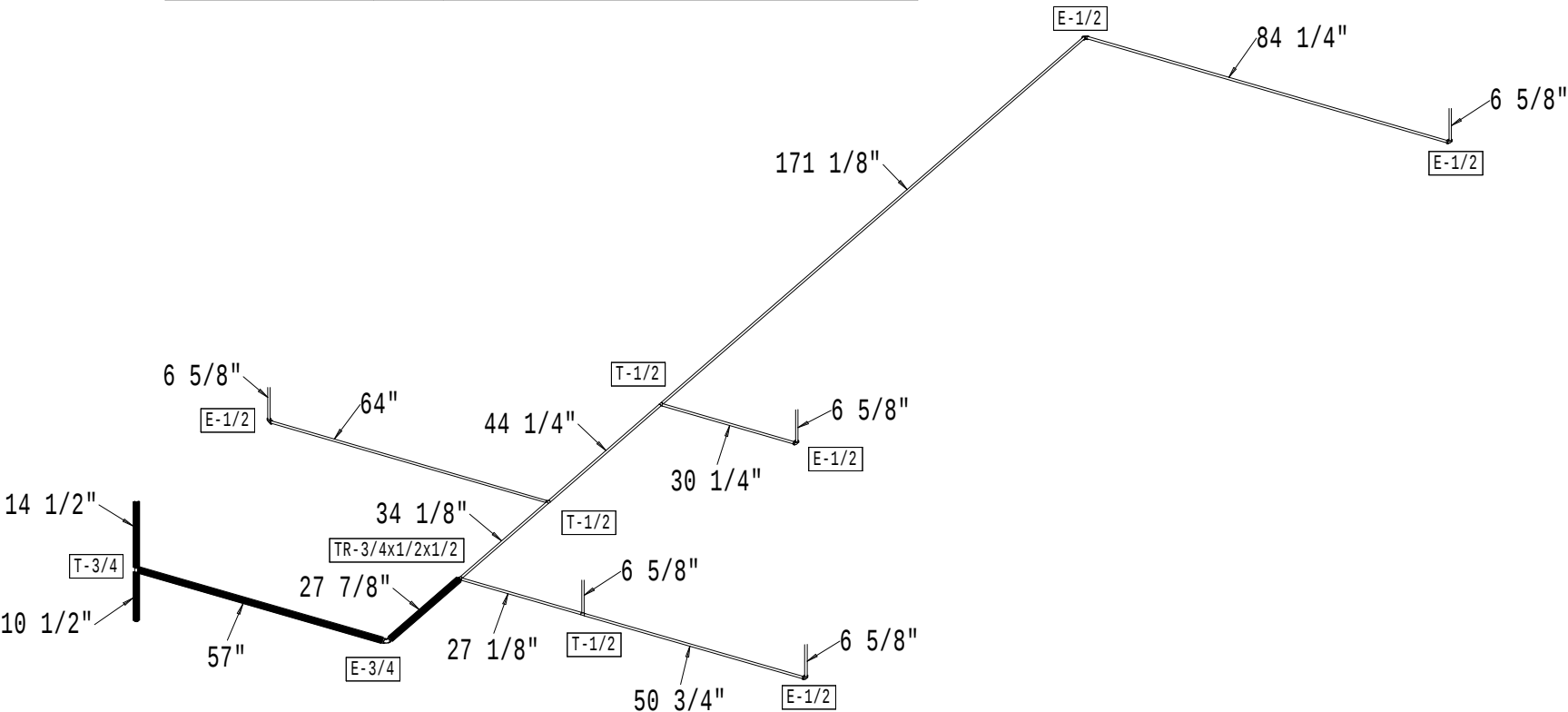
COLD WATER PLUMBING
