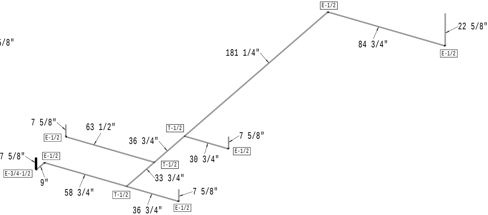
HOT WATER PLUMBING
