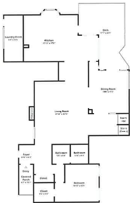
FLOOR 1 ENTRY LEVEL
