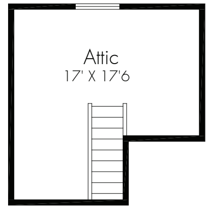
Upper Level
