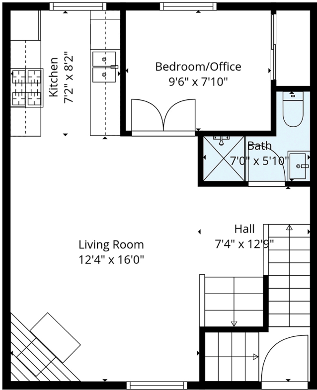
1st Floor
