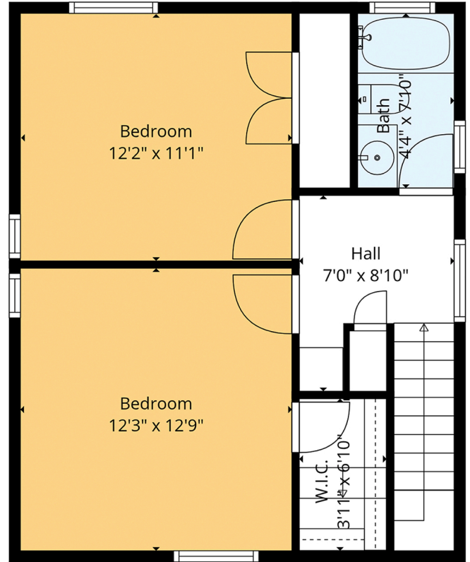
2nd Floor
