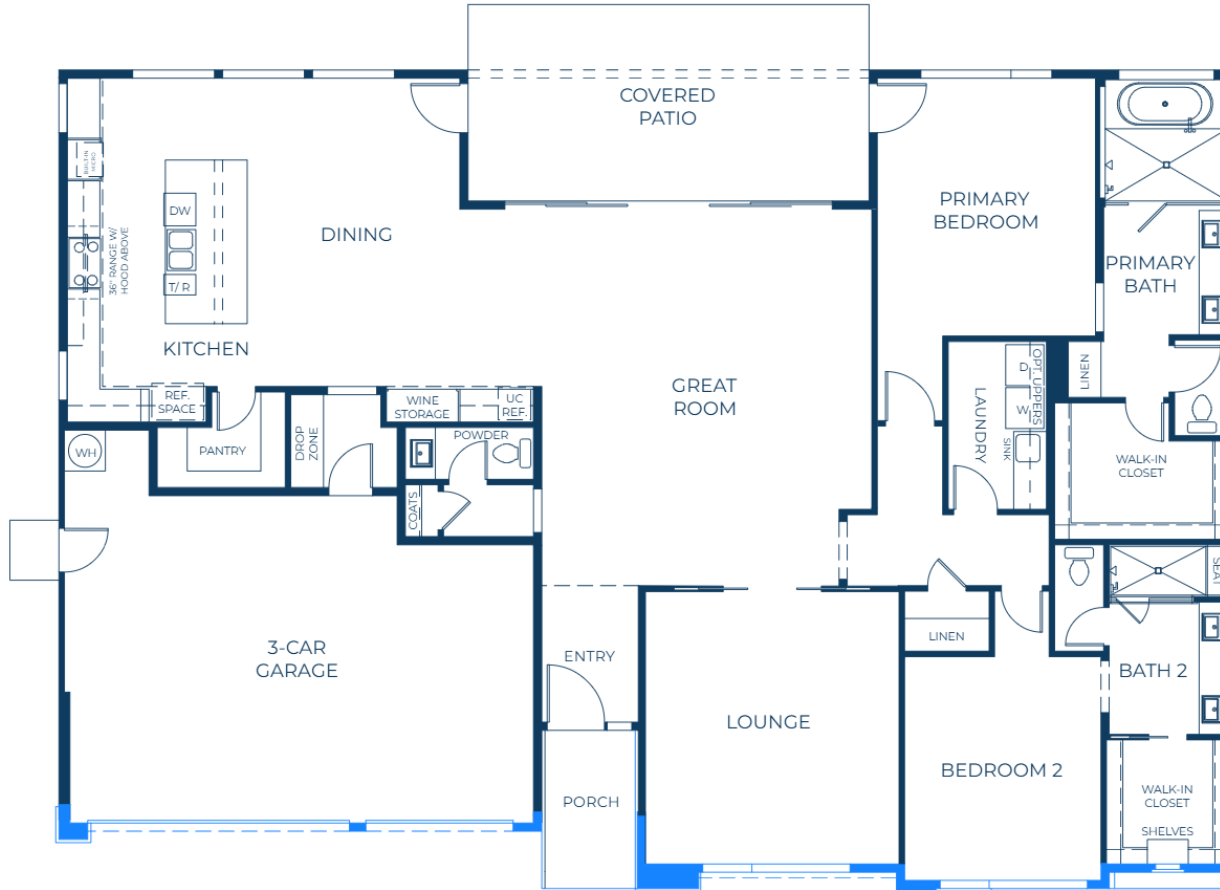
ELEVATION B FLOOR PLAN
