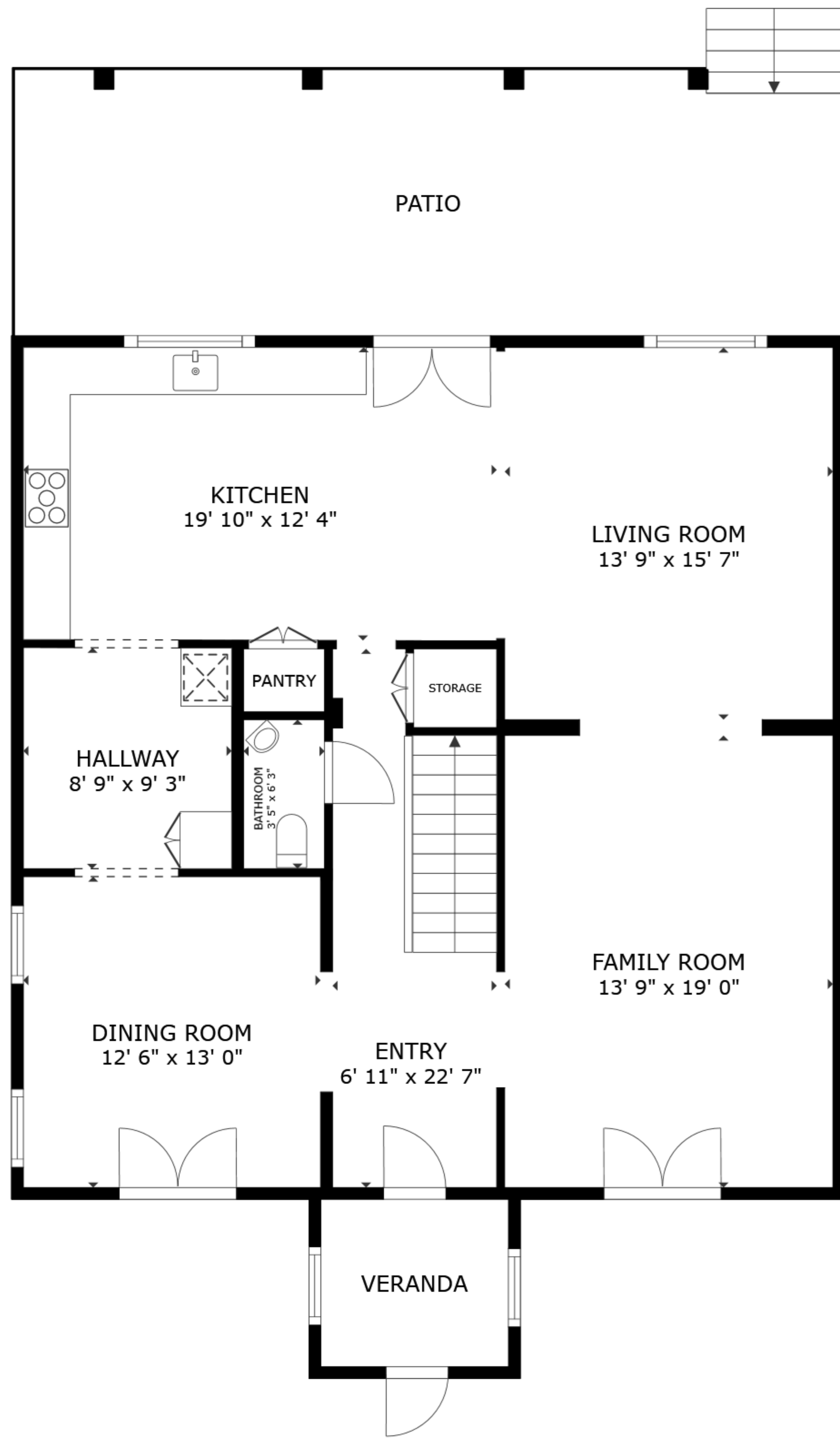
FLOOR 1
