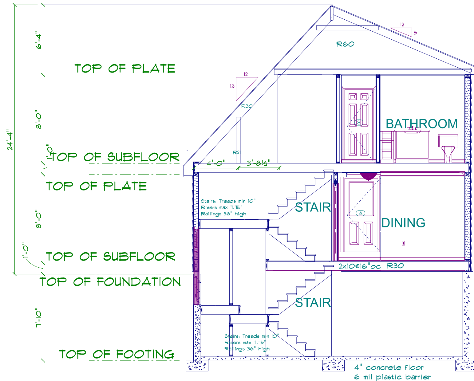
Cross Section
