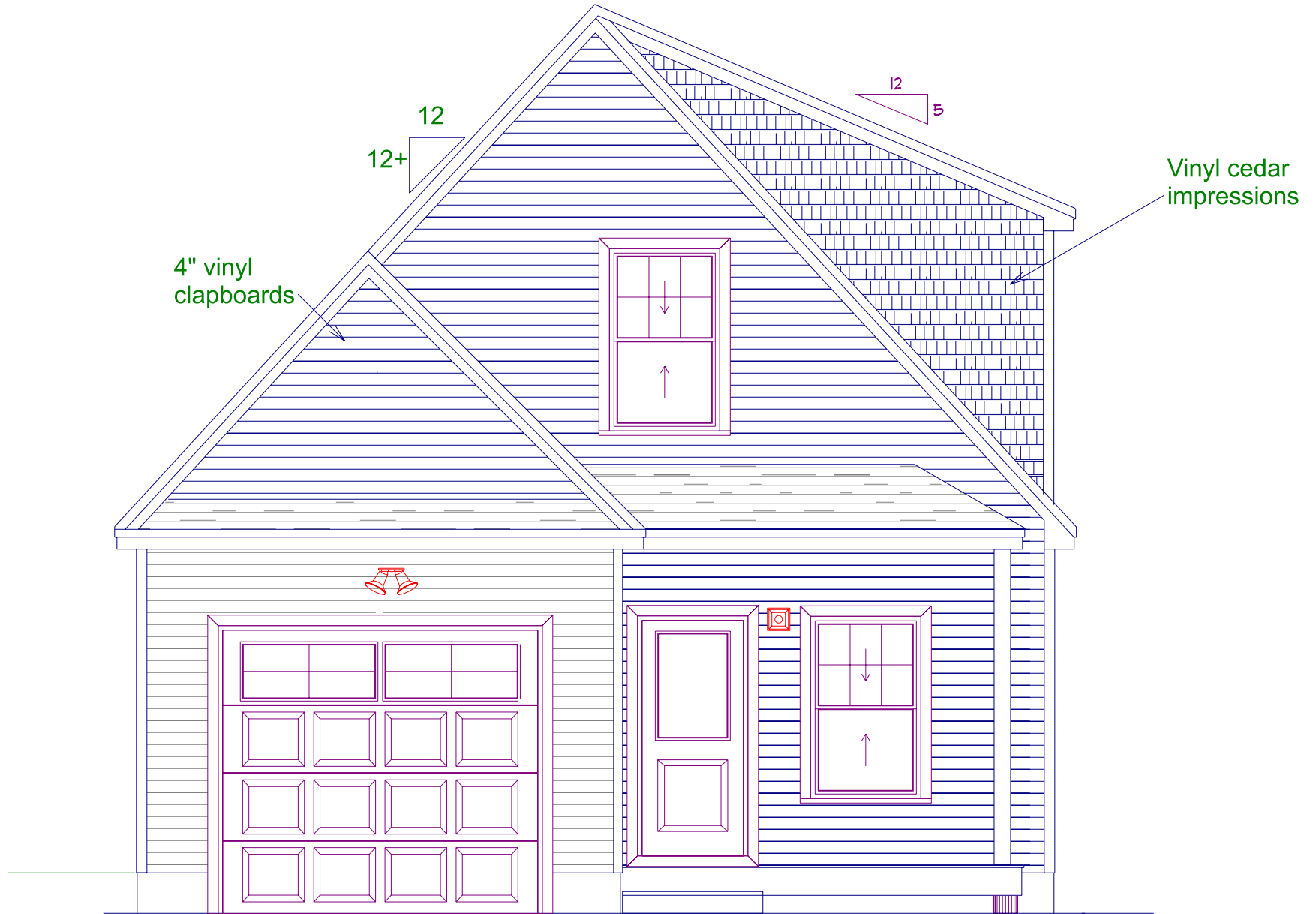
Front Elevation
