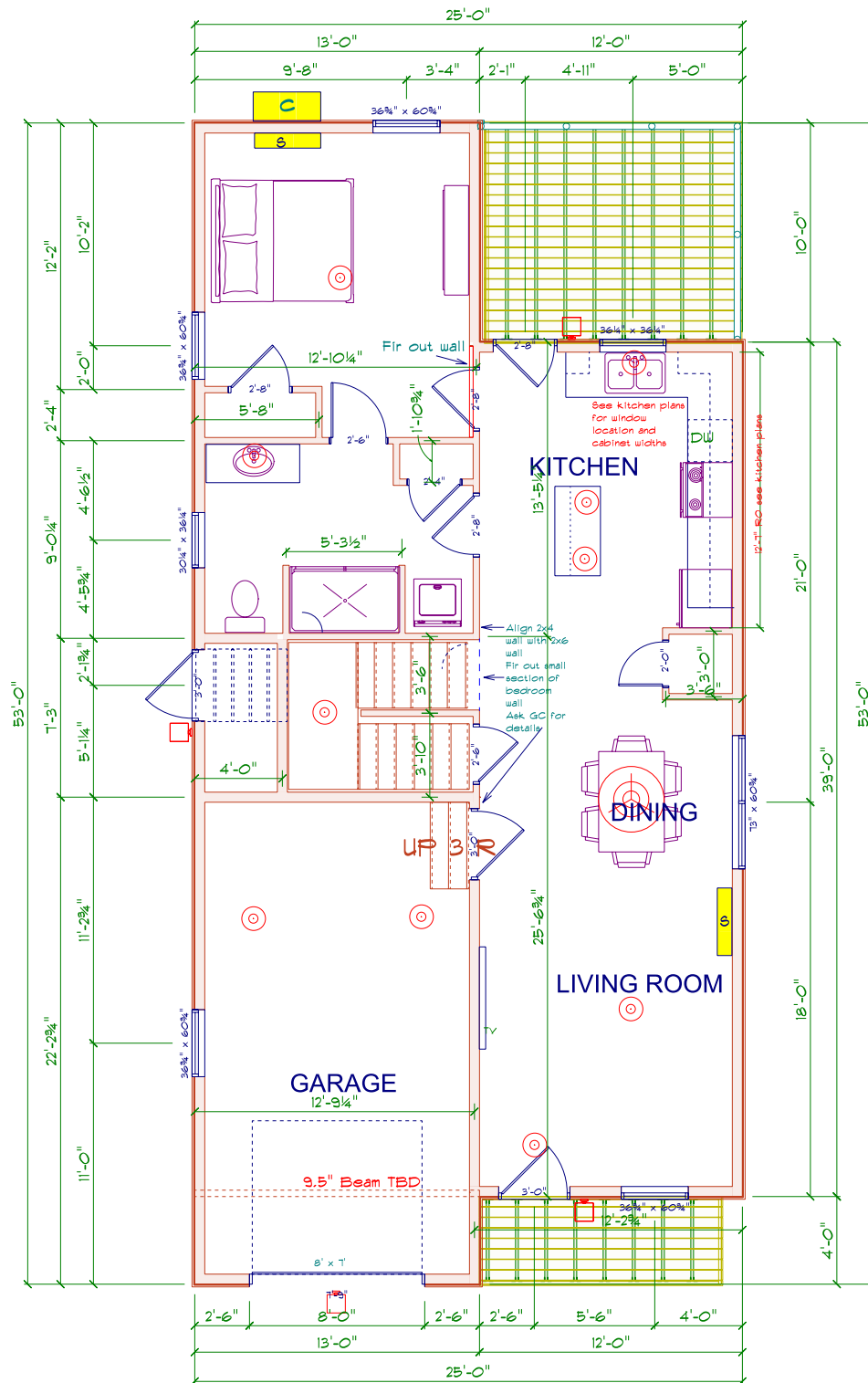
Main Floor
