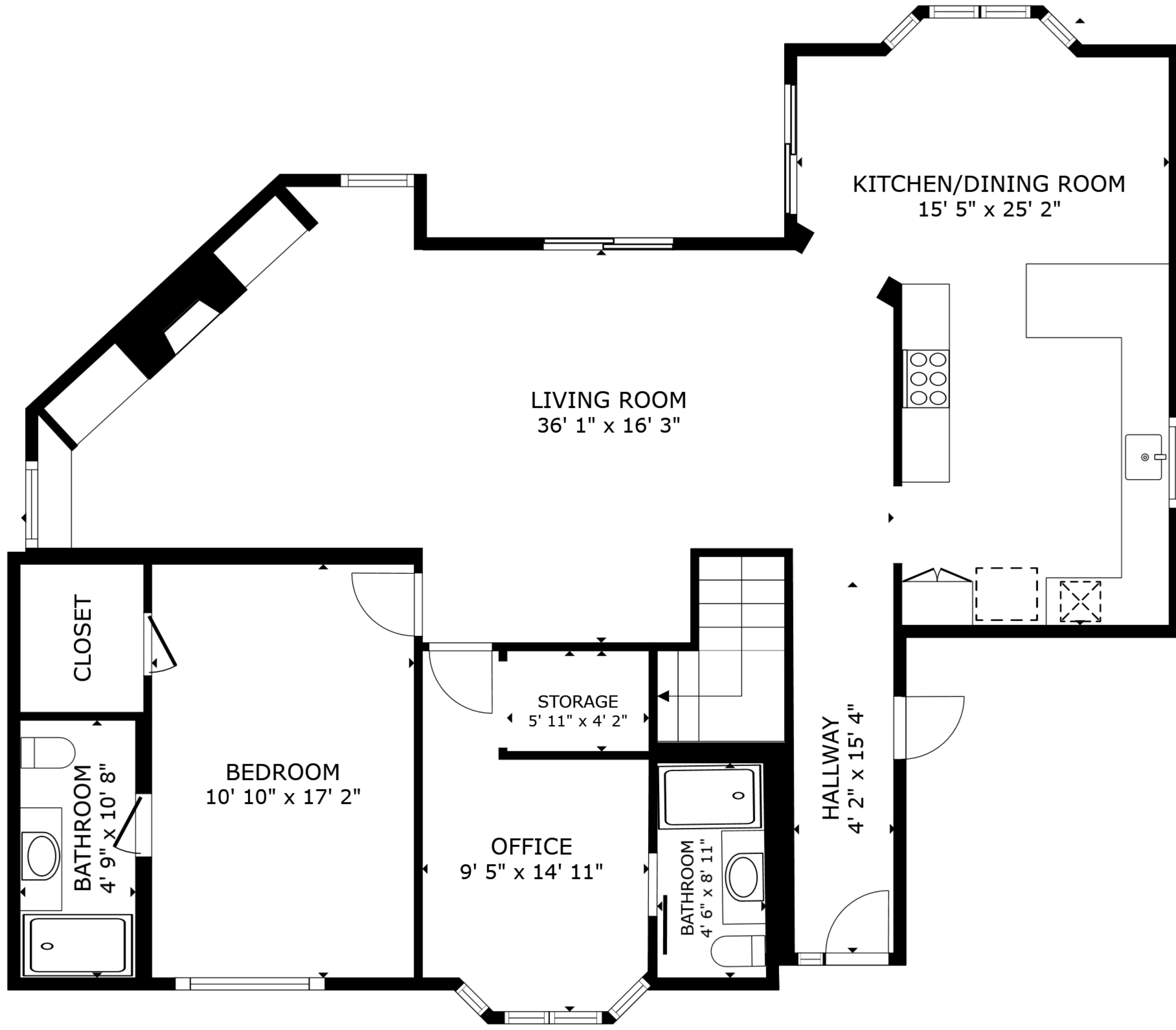
FLOOR 1
